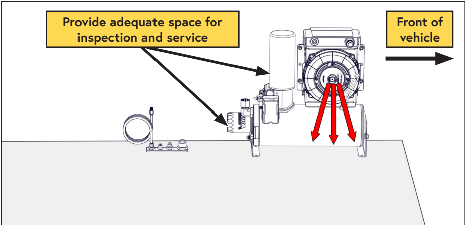
Figure 16 — WHASP ventilation
