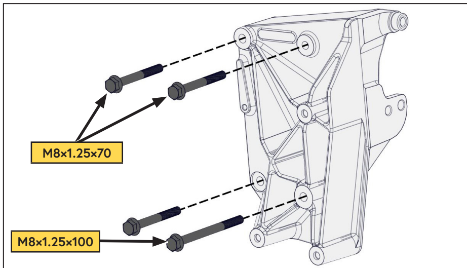
Figure 4 — VMAC Main bracket mount location
