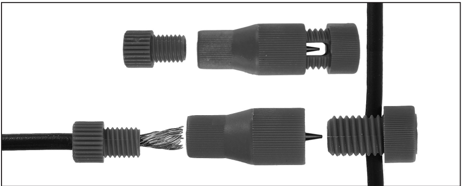
Figure 35 — Posi-Tap wire connector
