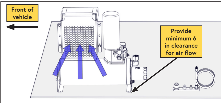
Figure 17 — WHASP ventilation
