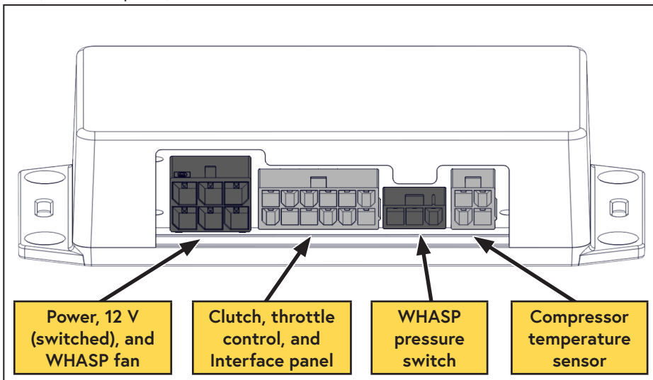
Figure 37 — Control module
