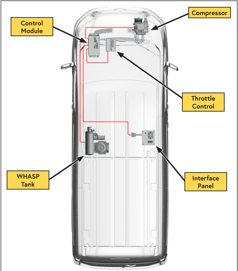
Figure 36 — General component overview (Actual installation locations may vary)
