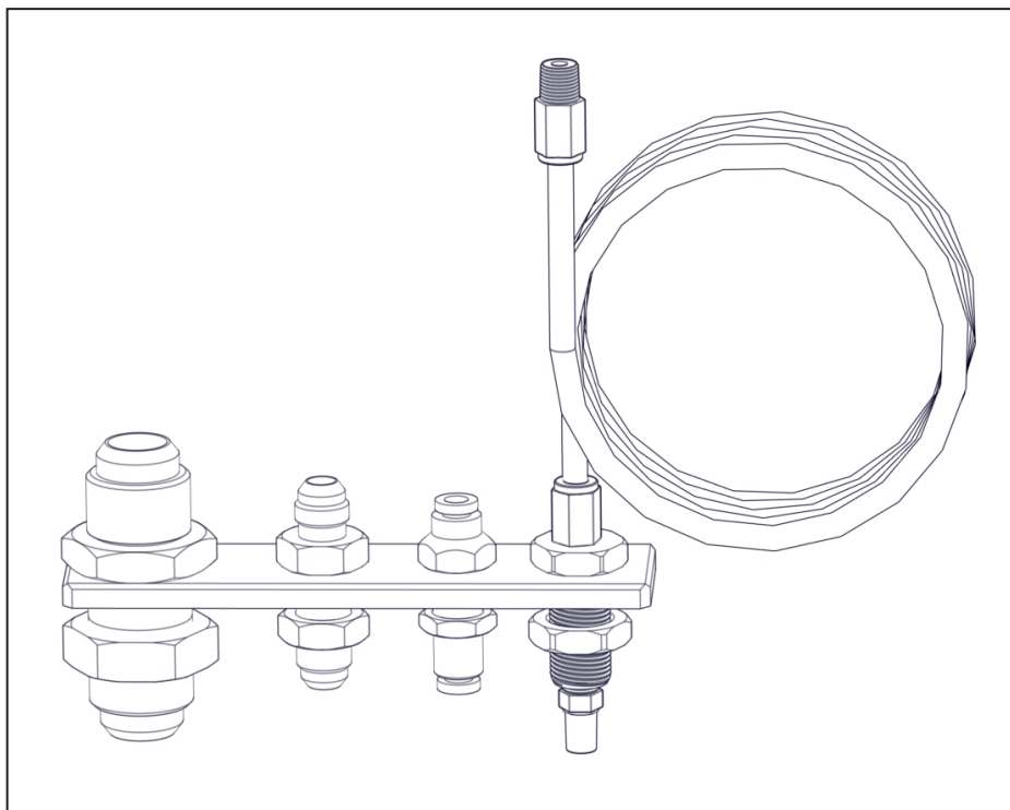
Figure 18 — Bulkhead fittings (A700224 Remote Muffler accessory shown)
