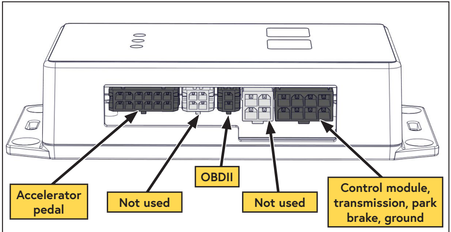
Figure 39 — VMAC digital throttle control
