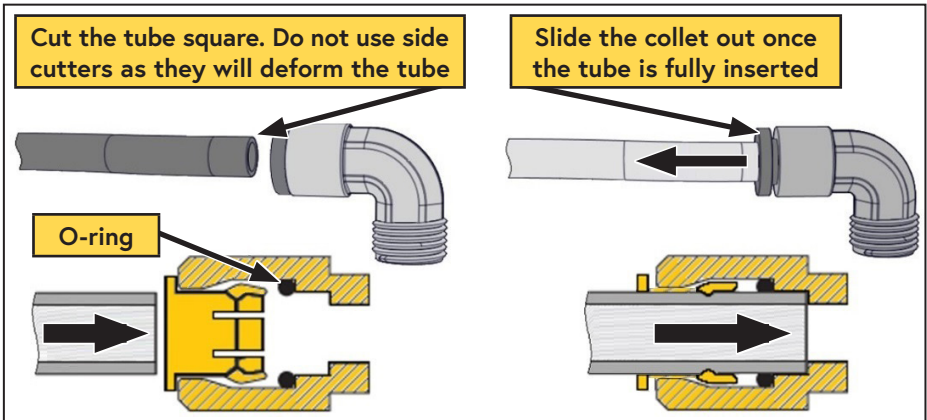
Figure 22 — Push-to-connect fittings
