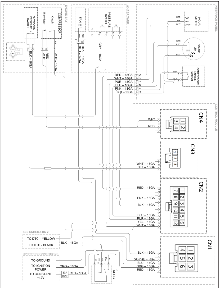
Figure 41 — Electrical schematic 1
