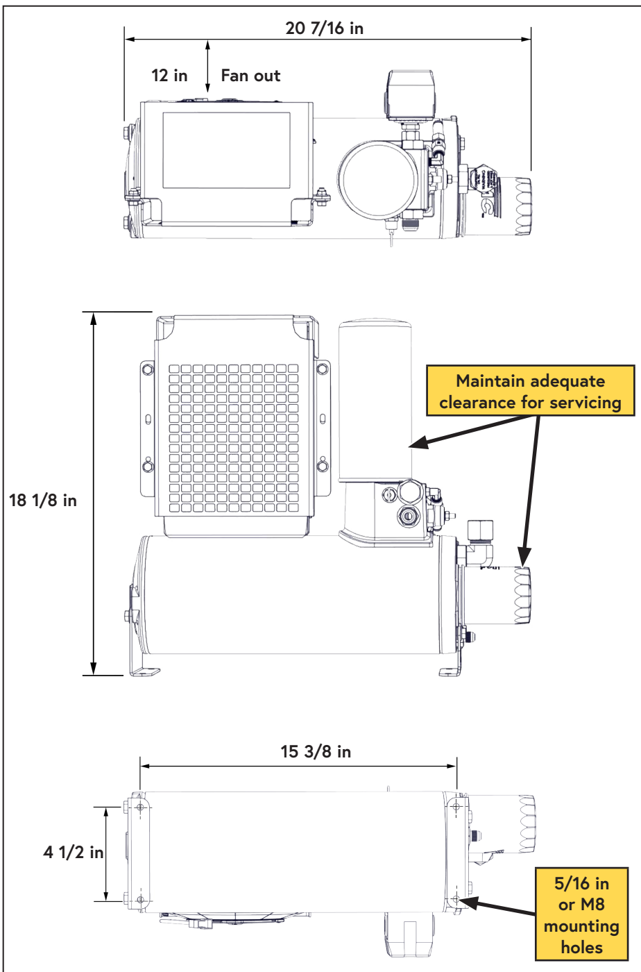
Figure 15 — Minimum WHASP Tank mounting clearances
