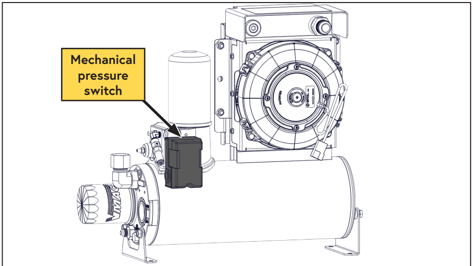
Figure 40 — WHASP Tank pressure switch
