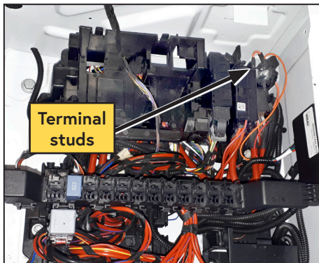
Figure 44 — Electrical access point
