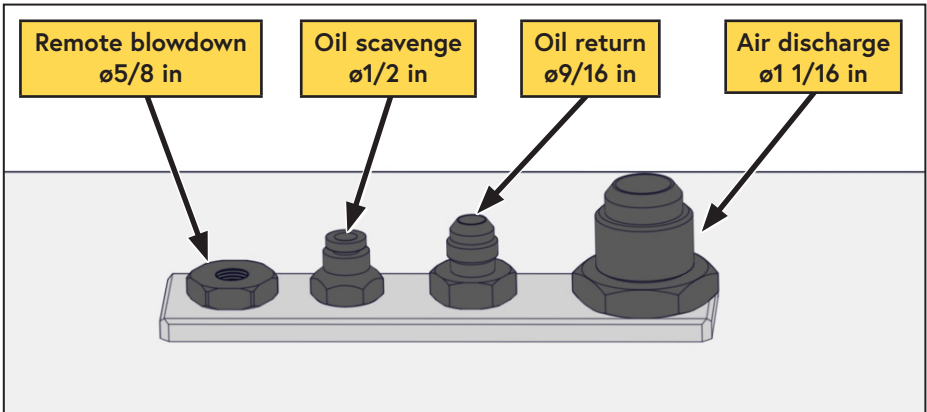
Figure 19 — Bulkhead fitting holes
