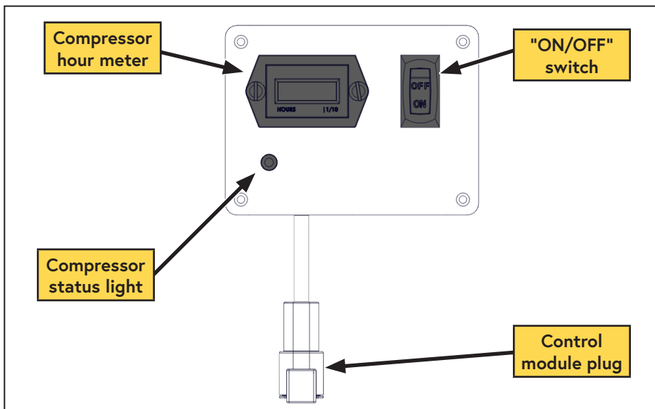
Figure 38 — Interface panel
