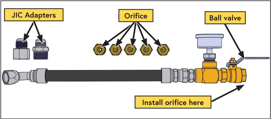
Figure 72 — A700052 VMAC Air Test Tool
