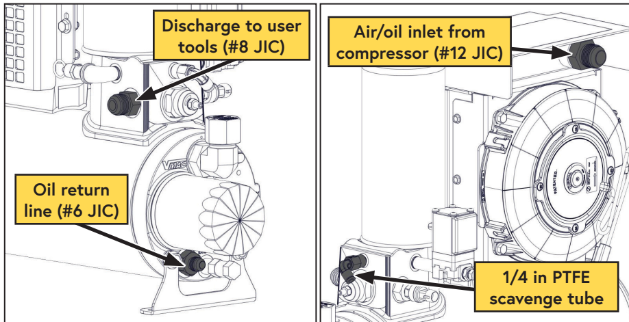
Figure 32 — WHASP Tank connections
