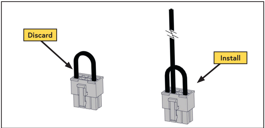
Figure 51 — Manual park brake 8 pin connector
