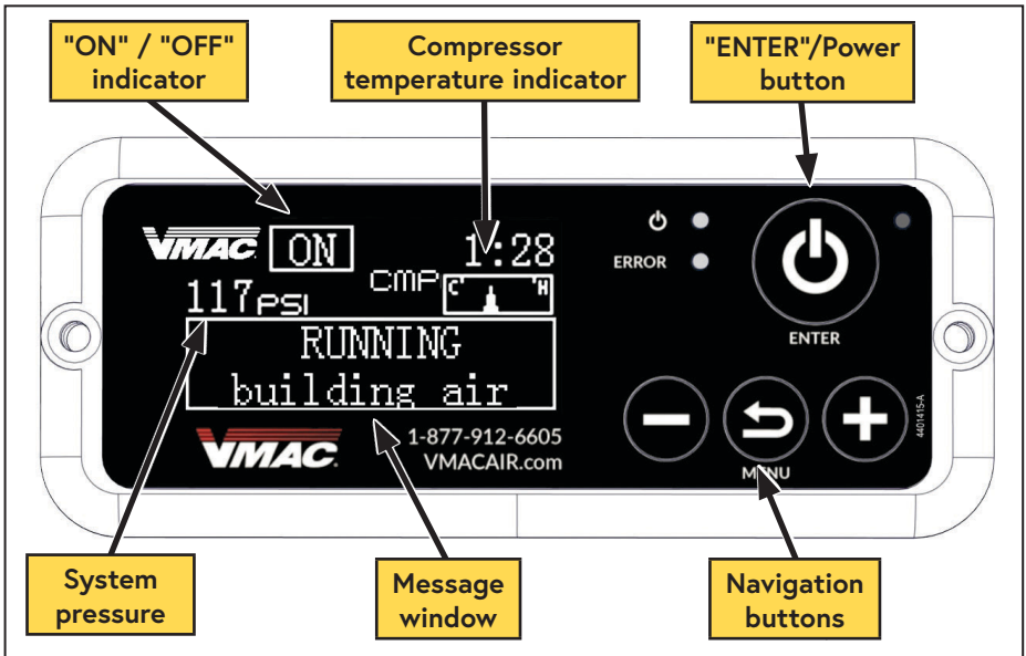
Figure 70 — Display box
