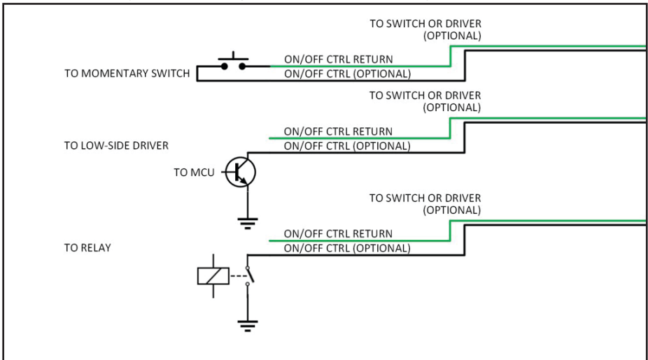
Figure 59 — Remote start integration
