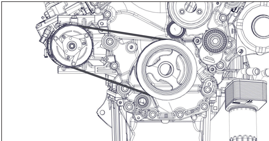
Figure 13 — Remove 4 rib belt
