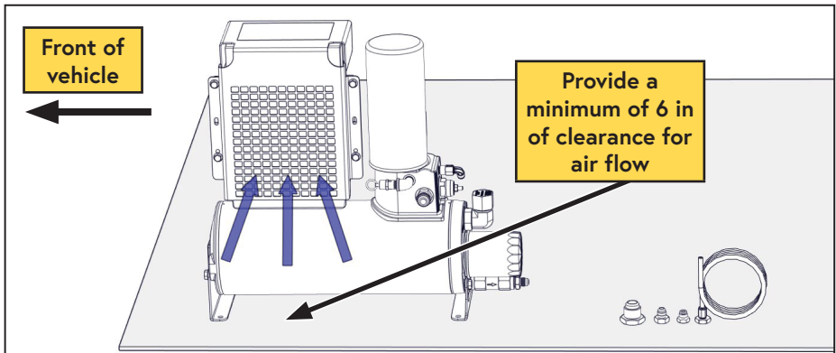
Figure 26 — WHASP ventilation
