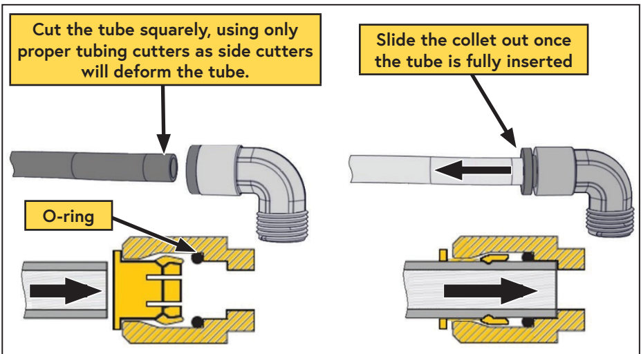
Figure 31 — Push-to-connect fittings
