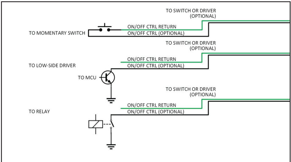
Figure 60 — Remote start integration
