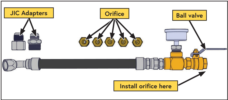
Figure 70 — A700052 VMAC Air Test Tool
