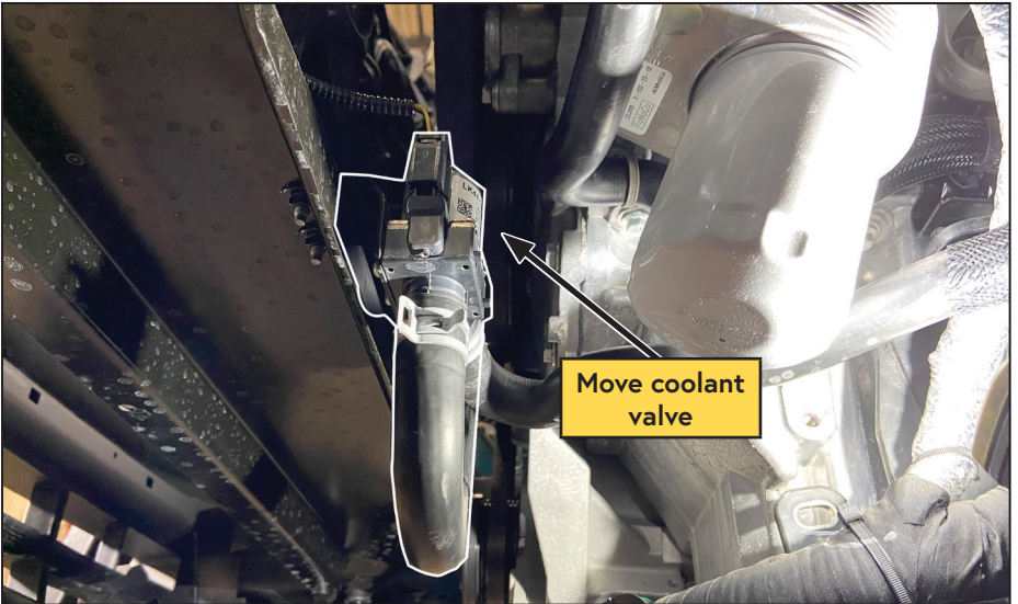
Figure 12 — Access tensioner bolt
