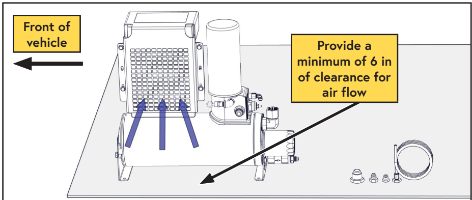
Figure 27 — WHASP ventilation
