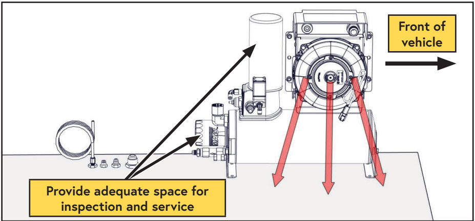
Figure 26 — WHASP ventilation
