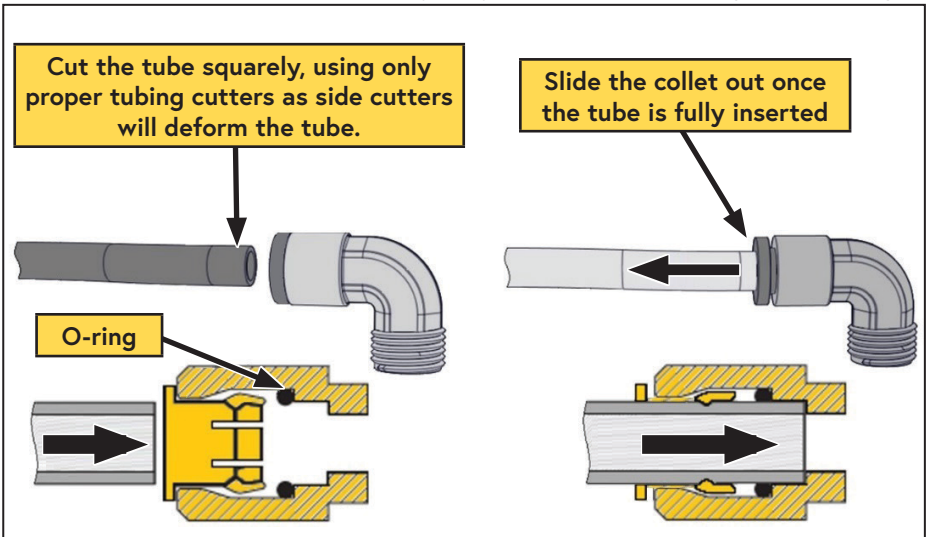
Figure 32 — Push-to-connect fittings
