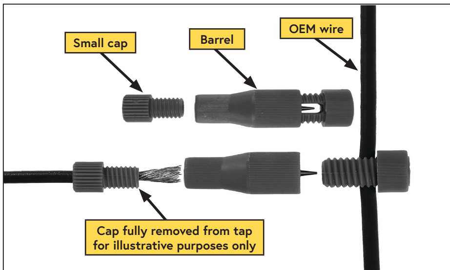
Figure 46 — Posi-Tap wire connector
