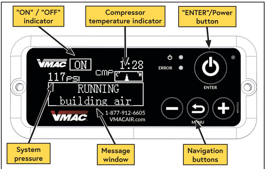
Figure 68 — Display box
