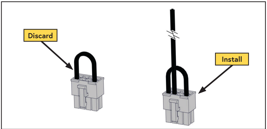
Figure 52 — Manual park brake 8 pin connector
