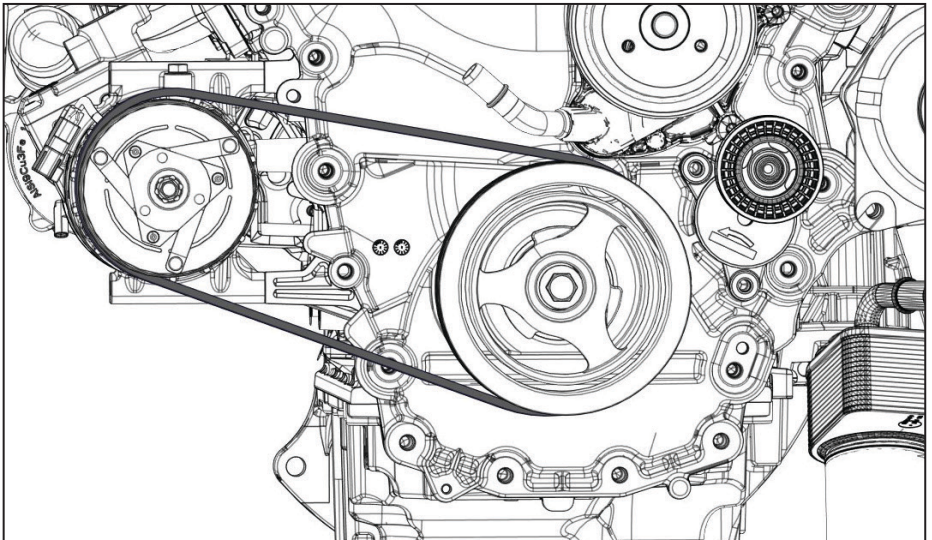
Figure 14 — Remove 4 rib belt
