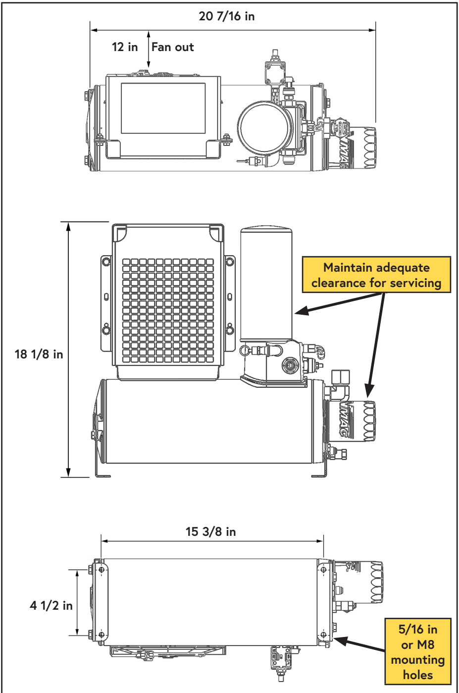
Figure 25 — Minimum WHASP Tank mounting clearances
