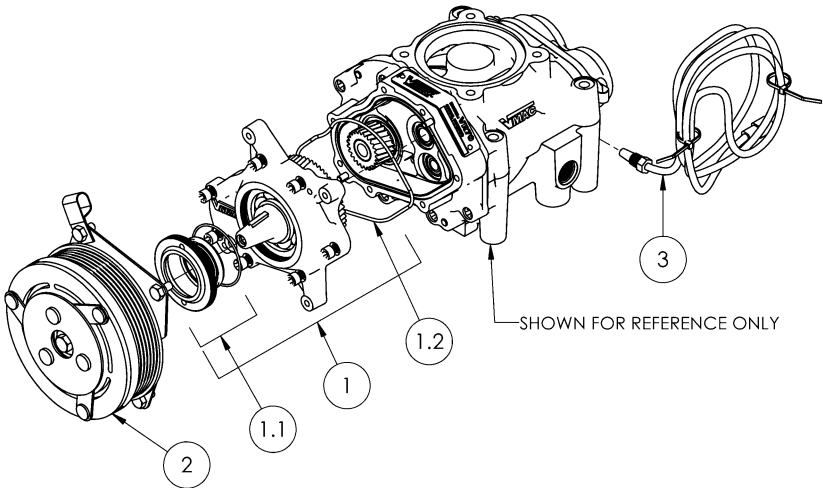
Figure 7 – Base Compressor Assembly
