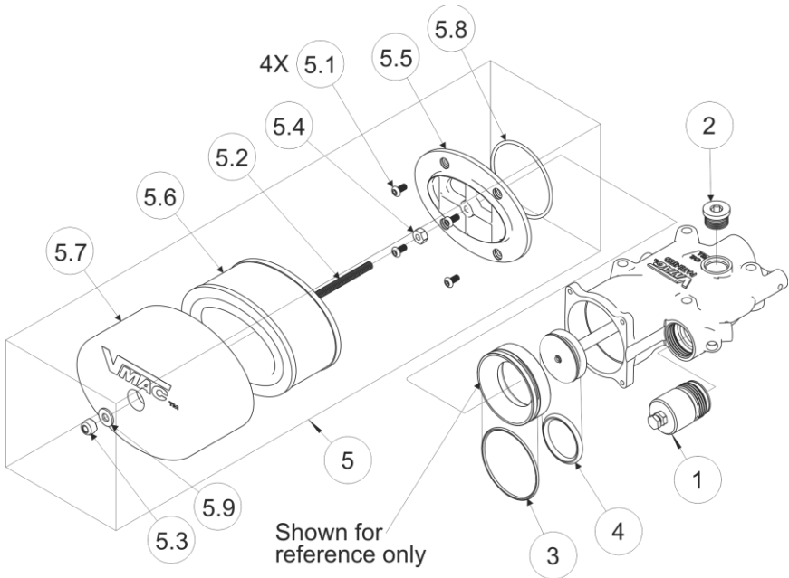
Figure 8 – Inlet Valve Sub Components
