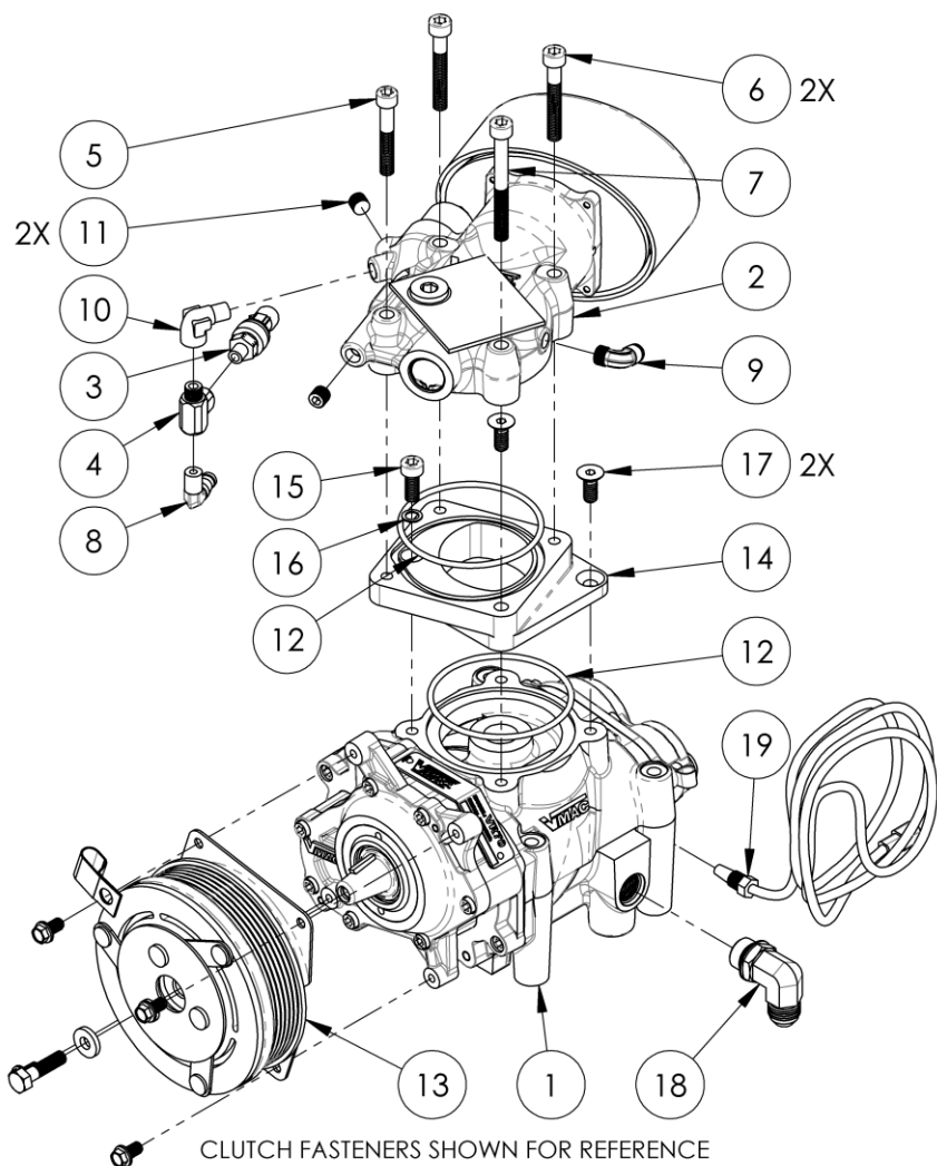
Figure 6 – Compressor Assembly
