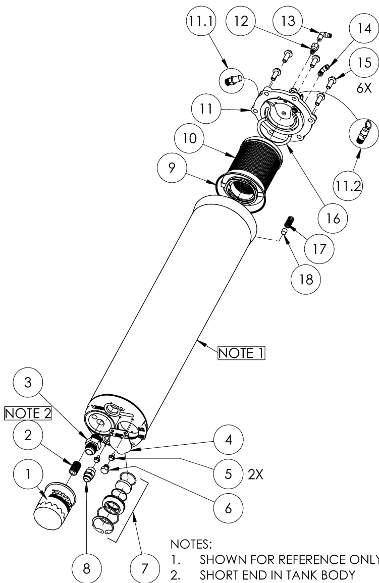
Figure 11 – VR70 Tank
