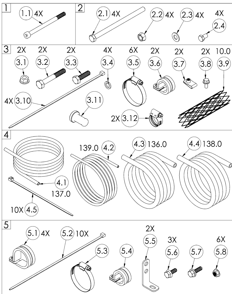
Figure 3 – Ford 6.7L VR70 Fastener Pack
