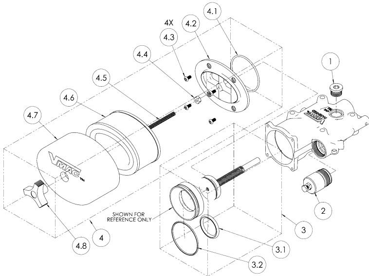
Figure 7 – Inlet Valve Sub Components
