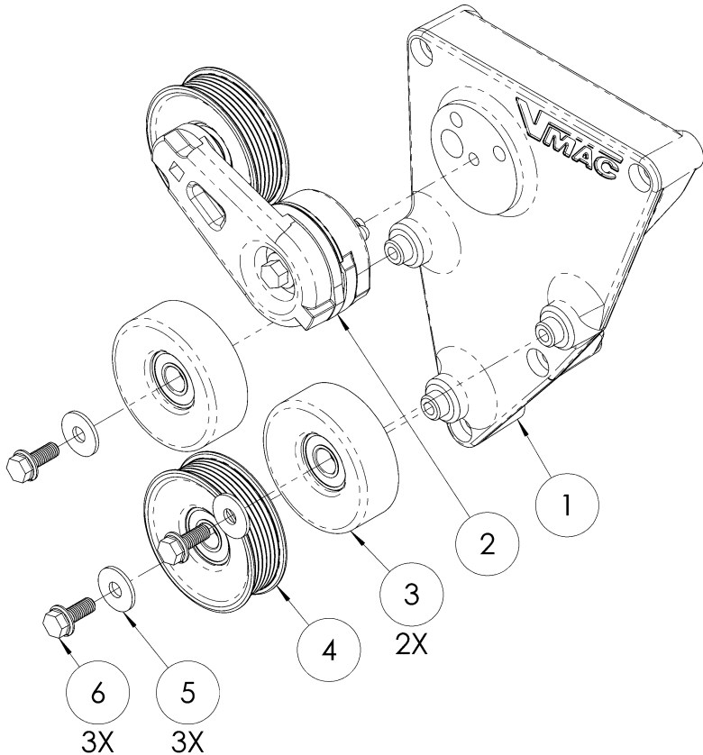
Figure 8 – FEAD Bracket Assembly
