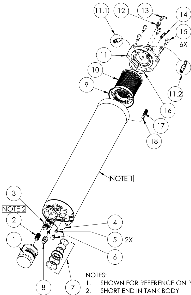
Figure 9 – VR70 Tank
