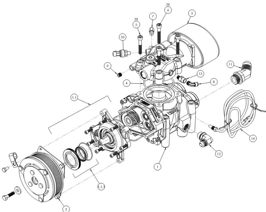
Figure 5 – Compressor Assembly
