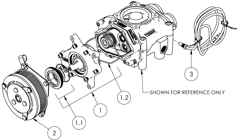
Figure 6 – Compressor Sub Components
