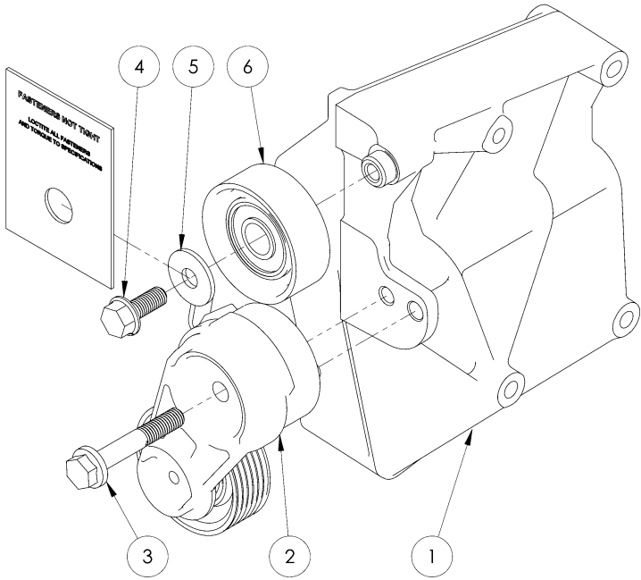
Figure 4 – Main Bracket Assembly
