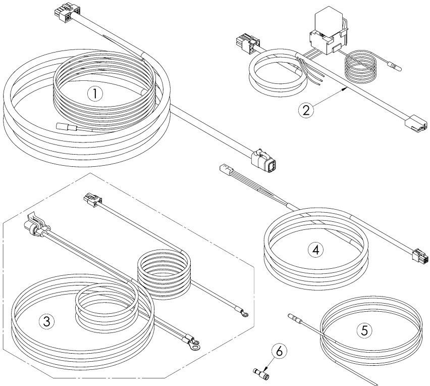
Figure 7 - Electrical Pack
