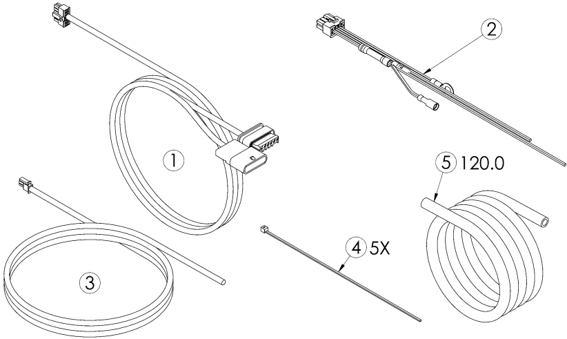
Figure 8 - Electrical Pack
