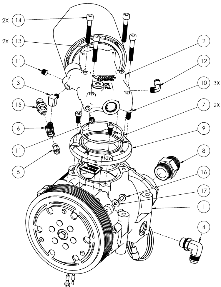
Figure 6 - Compressor Assembly
