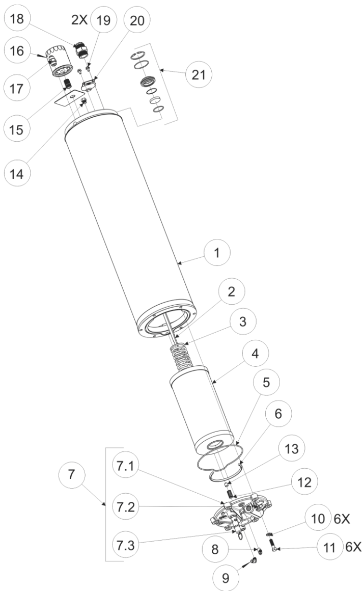
Figure 11 - VR150 Tank
