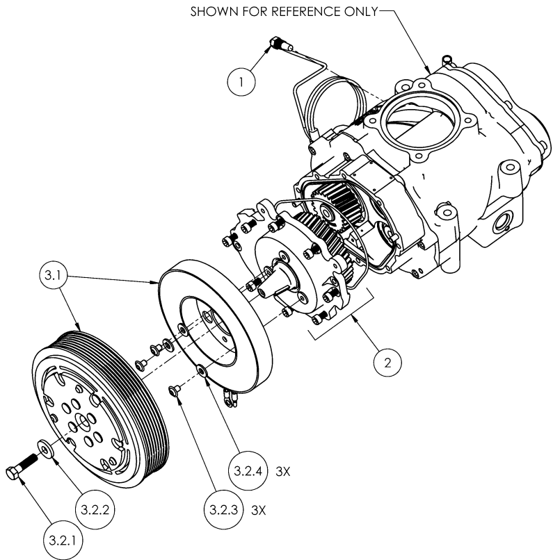
Figure 7 - Compressor Sub Components
