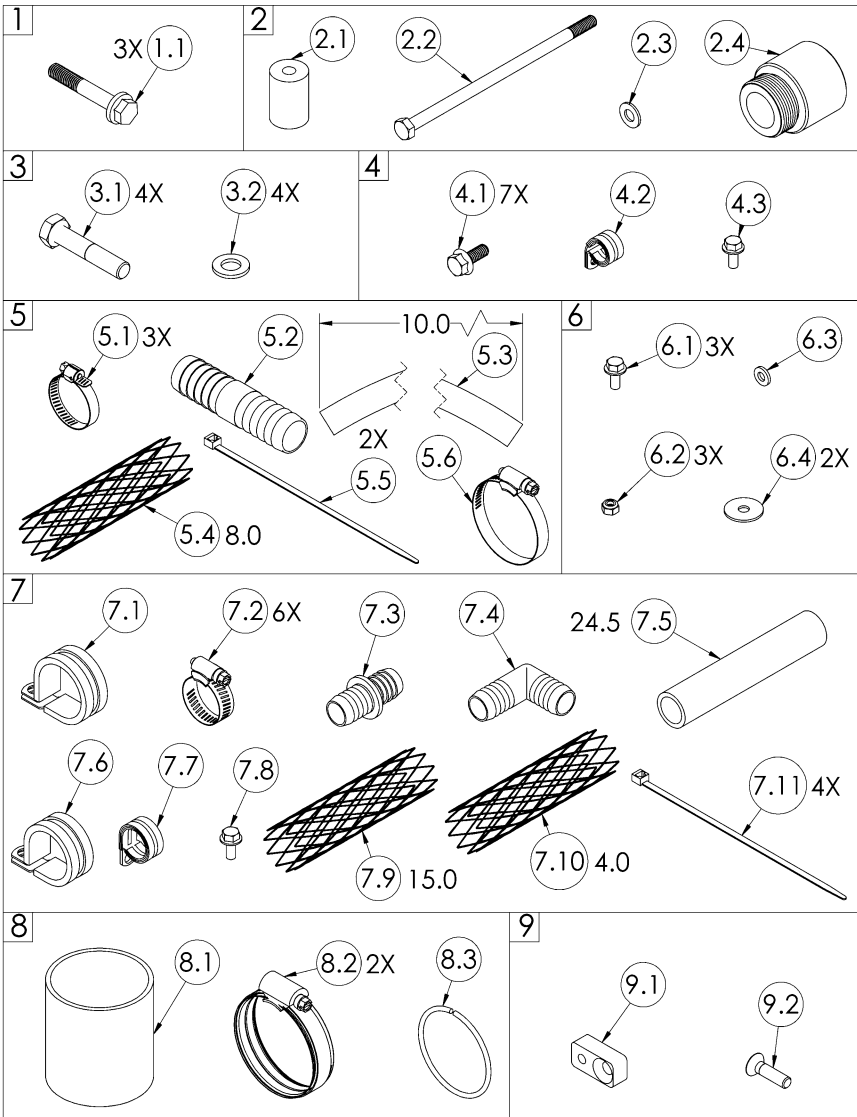
Figure 4 - Ford 6.7L VR70/150 Common Fastener Pack
