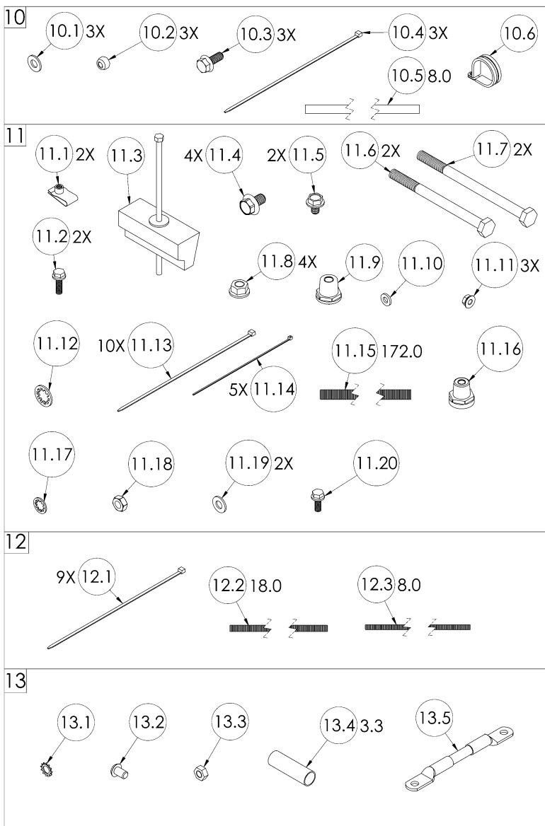
Figure 5 - Ford 6.7L VR70/150 Common Fastener Pack (cont'd)
