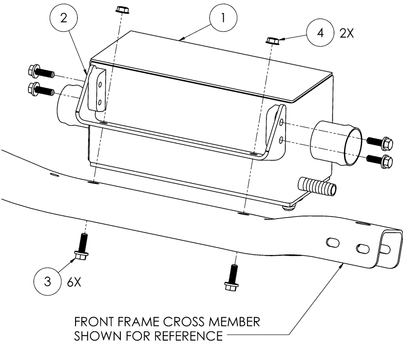
Figure 10 - Cooler Assembly
