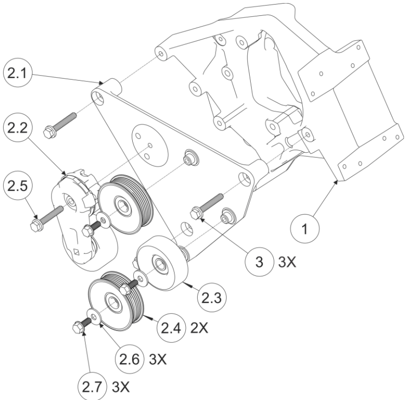
Figure 9 - FEAD and Main Bracket Assembly
