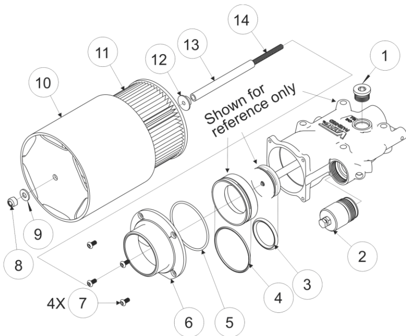
Figure 8 - Inlet Valve Sub Components
