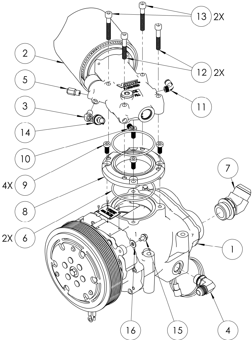
Figure 5 – Compressor Assembly
