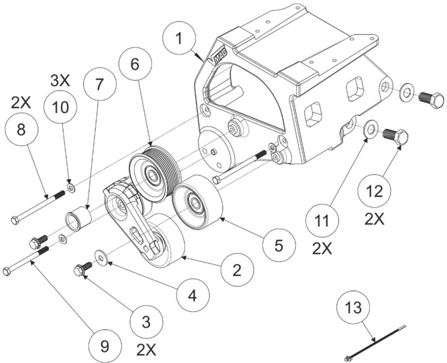
Figure 8 – Main Bracket Assembly
