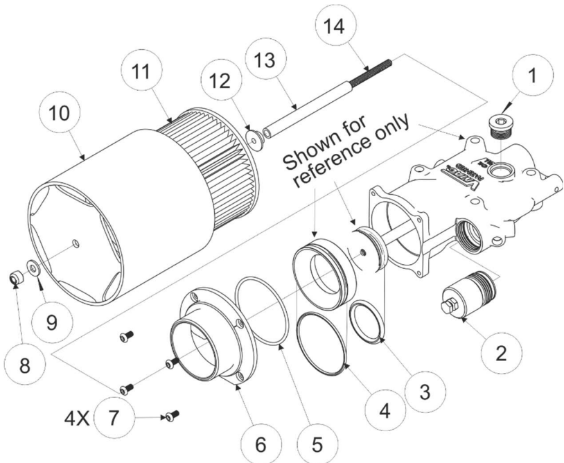
Figure 7 – Inlet Valve Sub Components
