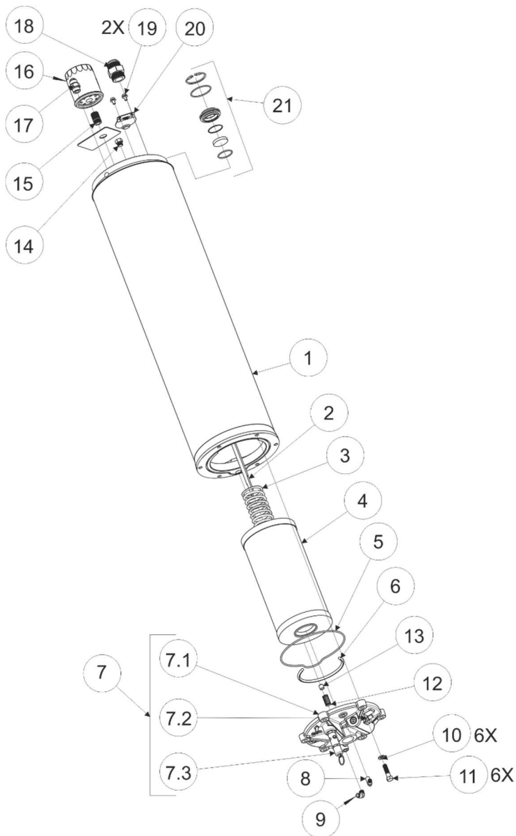
Figure 9 – VR150 Tank
