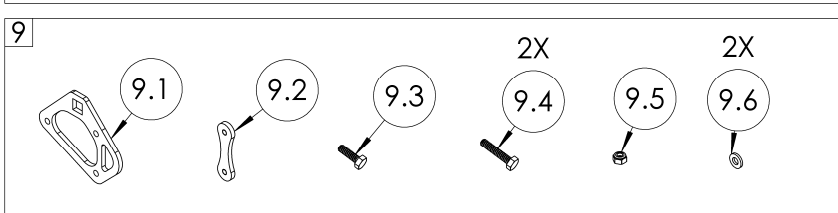
Figure 3 – Fastener Packs (CONTINUED)
