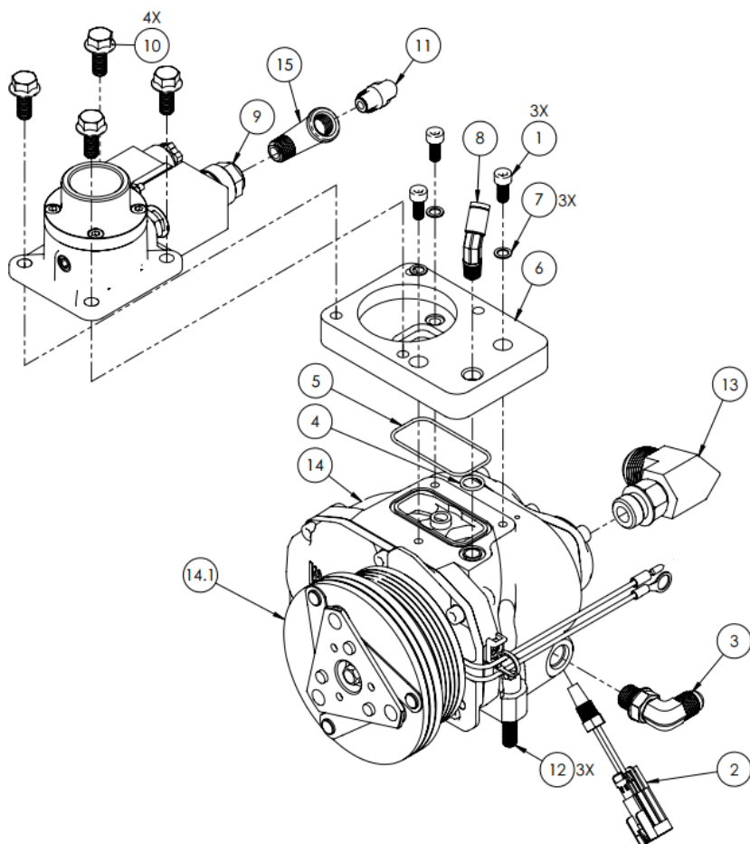
Figure 4 – Compressor Assembly
