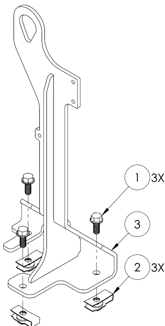
Figure 8 – Lifting Hook Assembly
