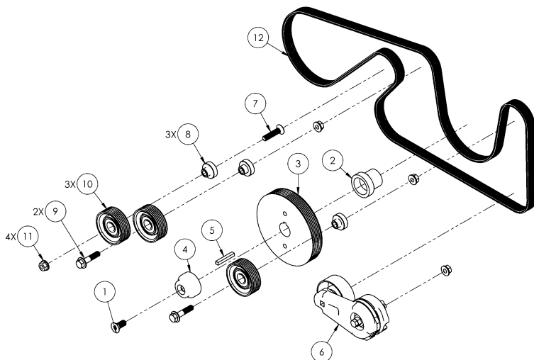
Figure 3 – Drive Assembly
