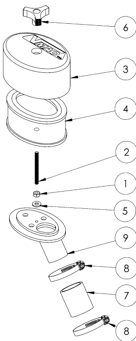
Figure 5 – Air Filter Assembly
