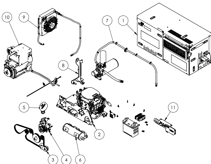
Figure 0 – Sub Assy Overview
