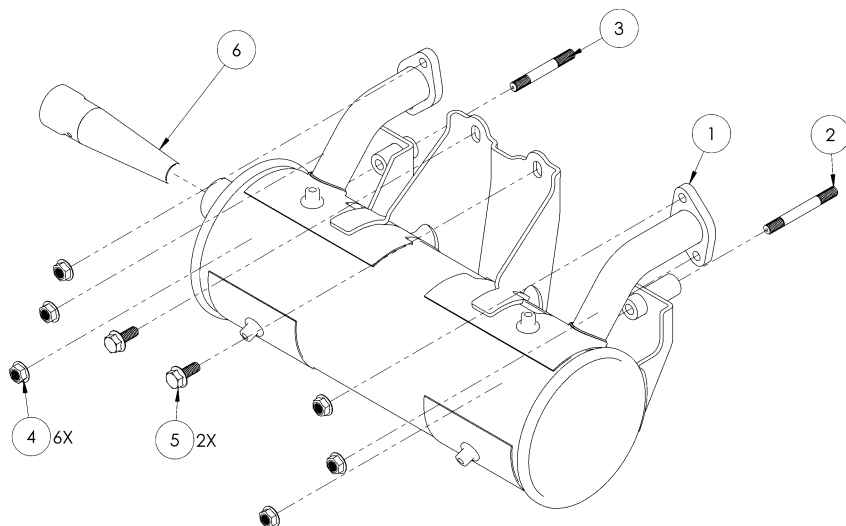
Figure 6 – Exhaust Assembly
