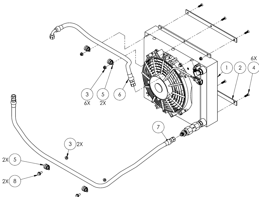
Figure 9 – Cooler Assembly, Complete
