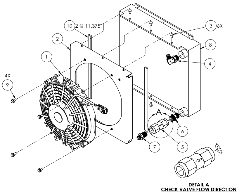
Figure 9.1 – Cooler Assembly Parts
