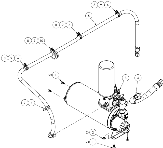
Figure 7 – AOST Assembly
