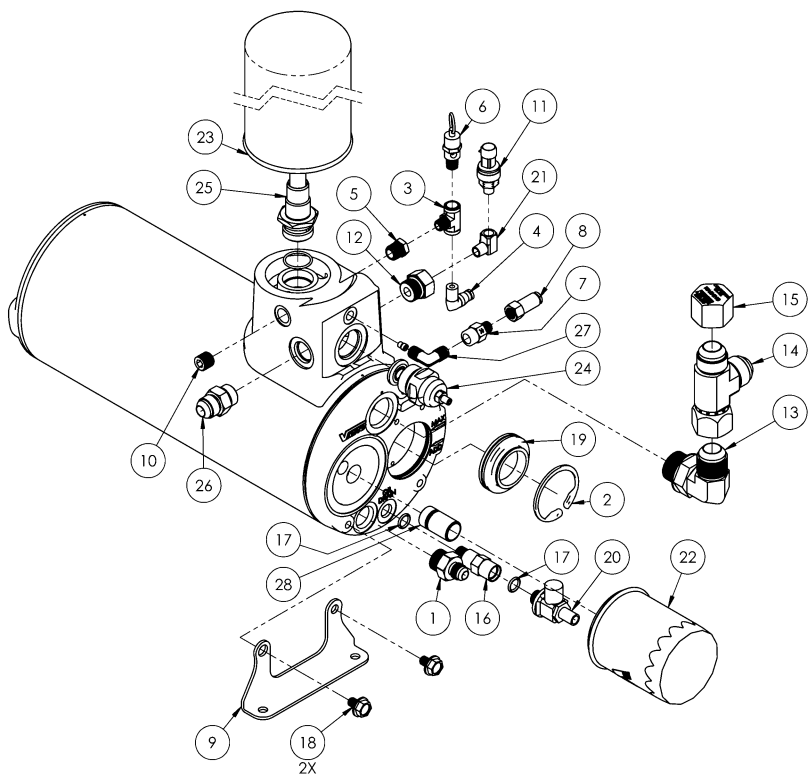
Figure 7.1 – AOST Assembly Parts
