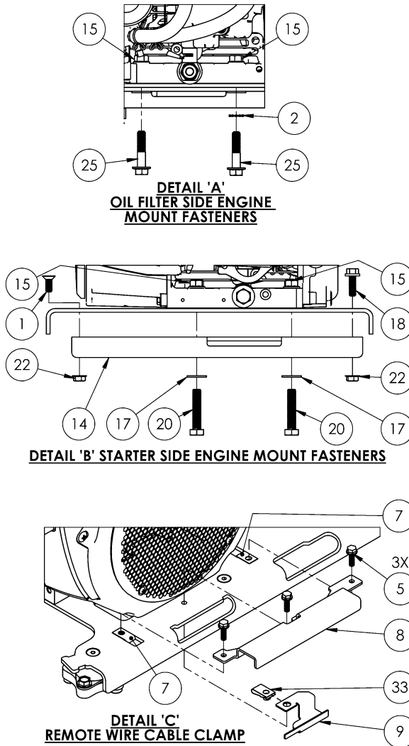
Figure 2.1 – Engine Assembly
