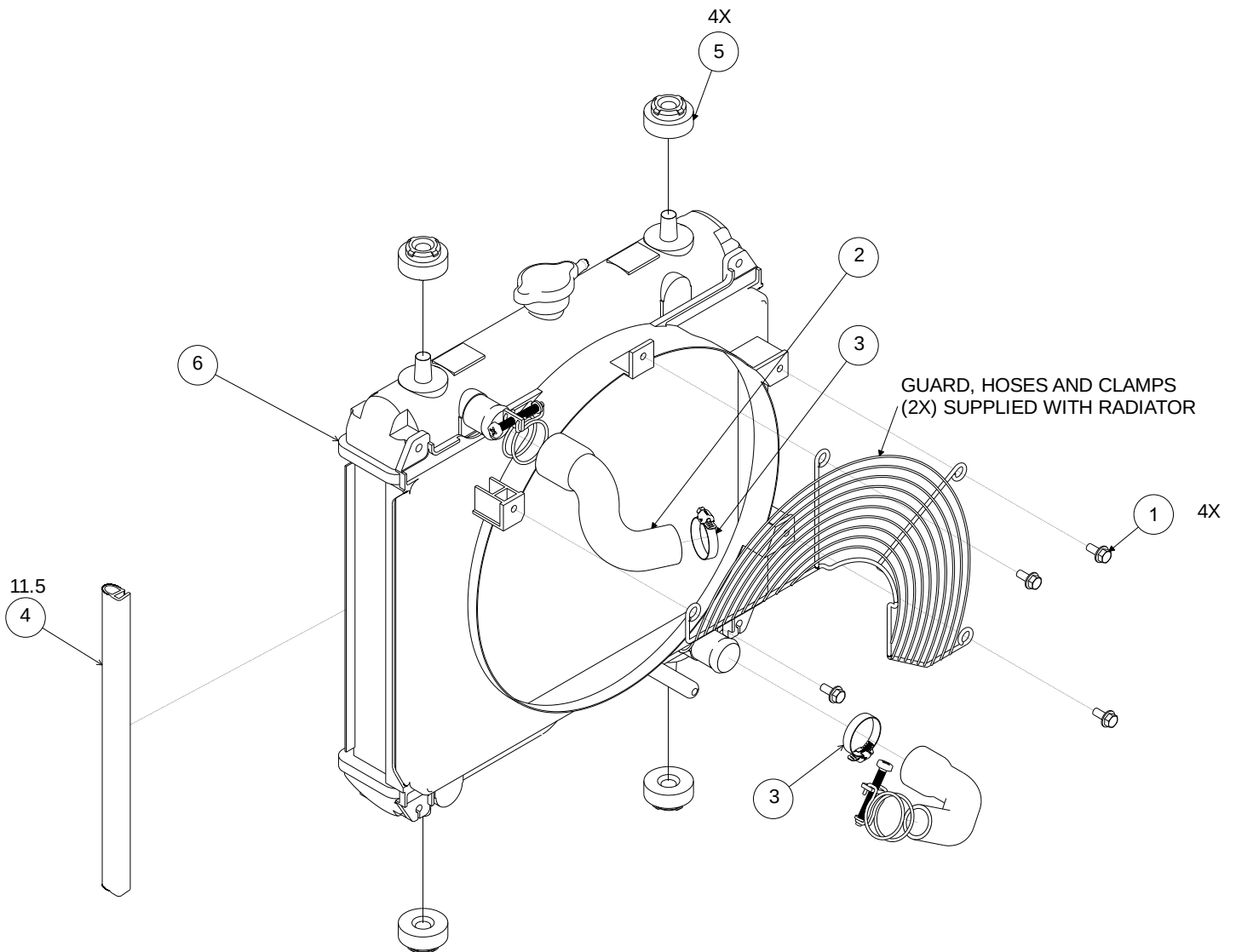
Figure 3 – Radiator Assembly
