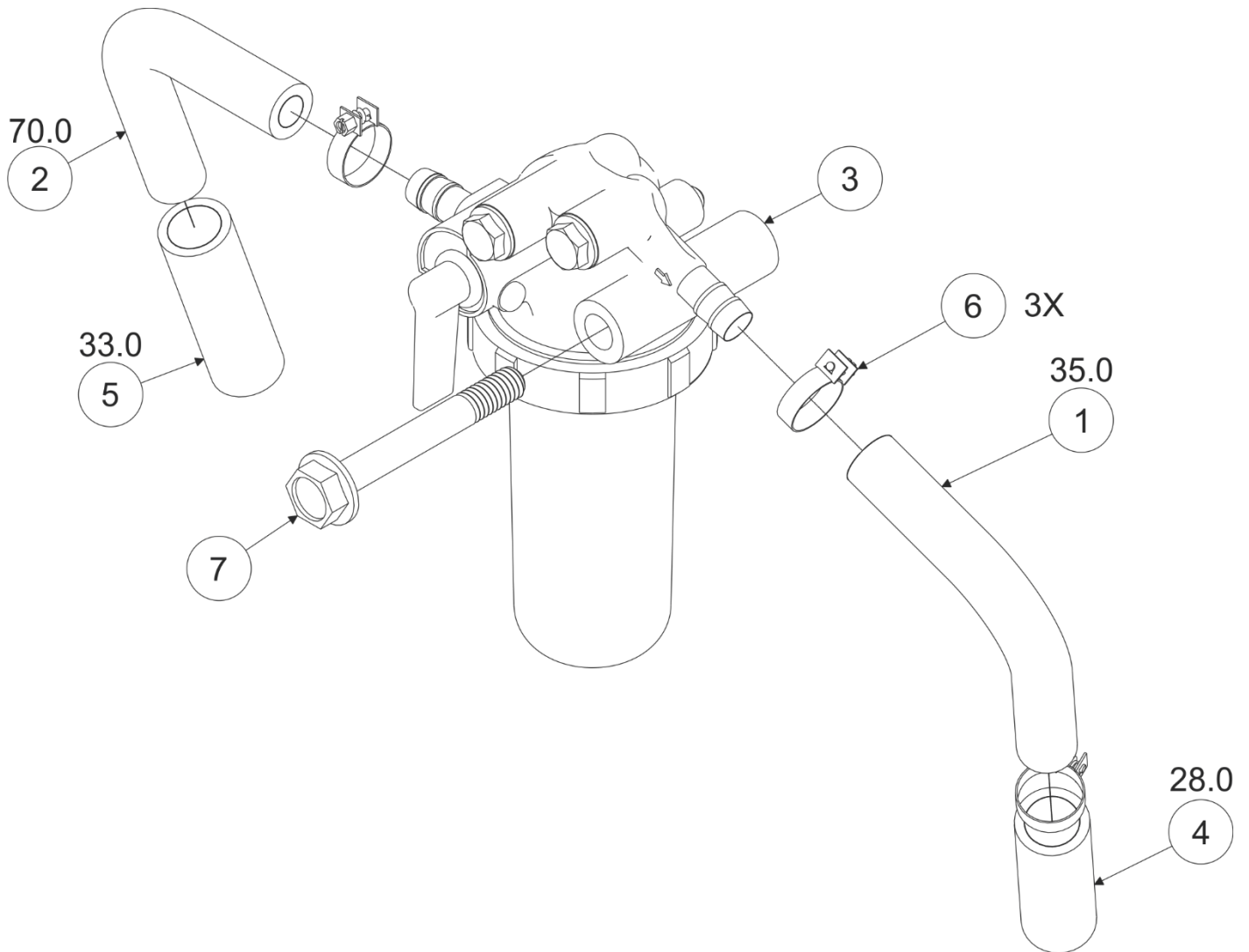
Figure 14 – Fuel Filter Assembly
