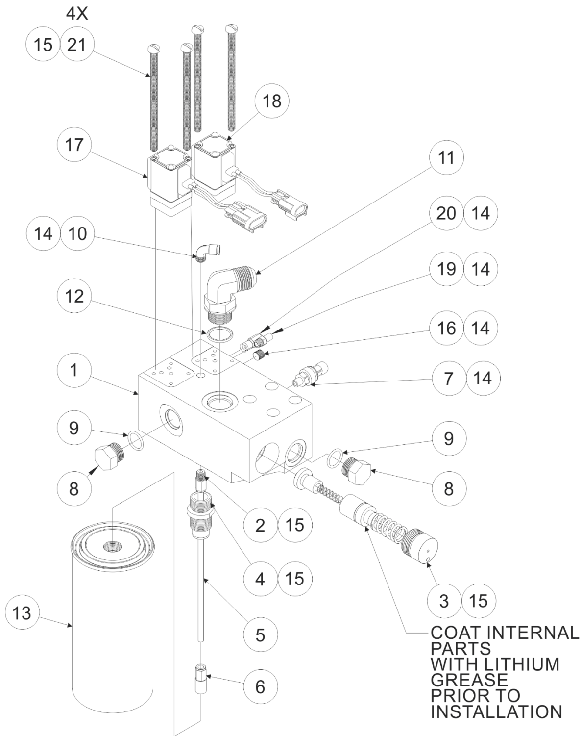
Figure 9 – Manifold Assembly
