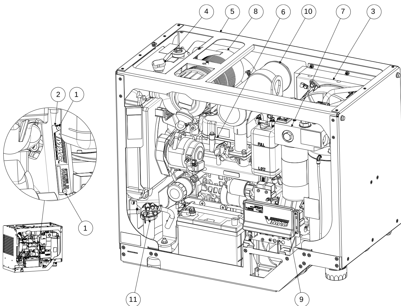
Figure 1 – Main Assembly
