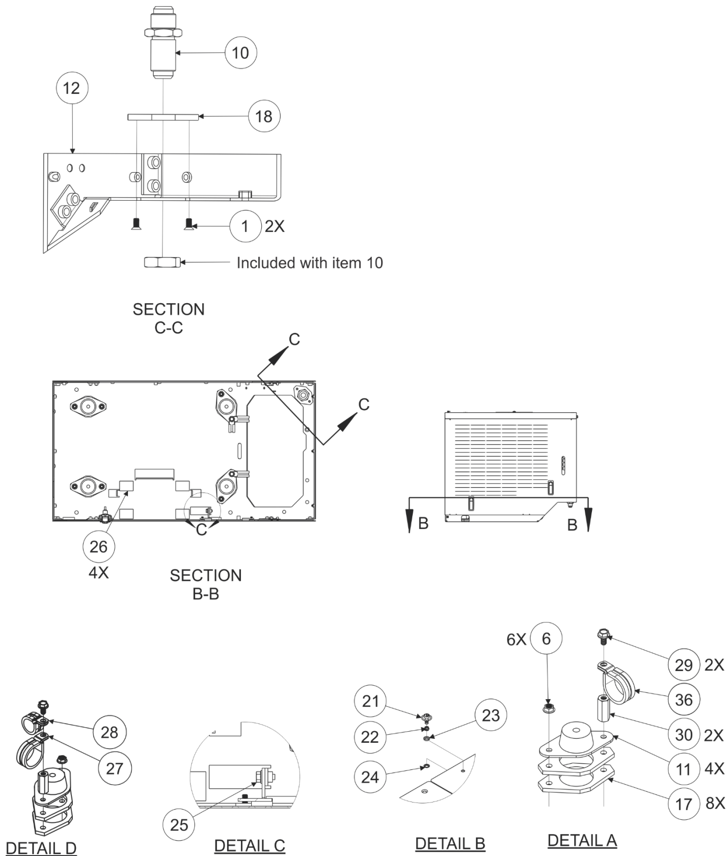
Figure 4.1 – Frame & Sheet Metal Assembly Details
