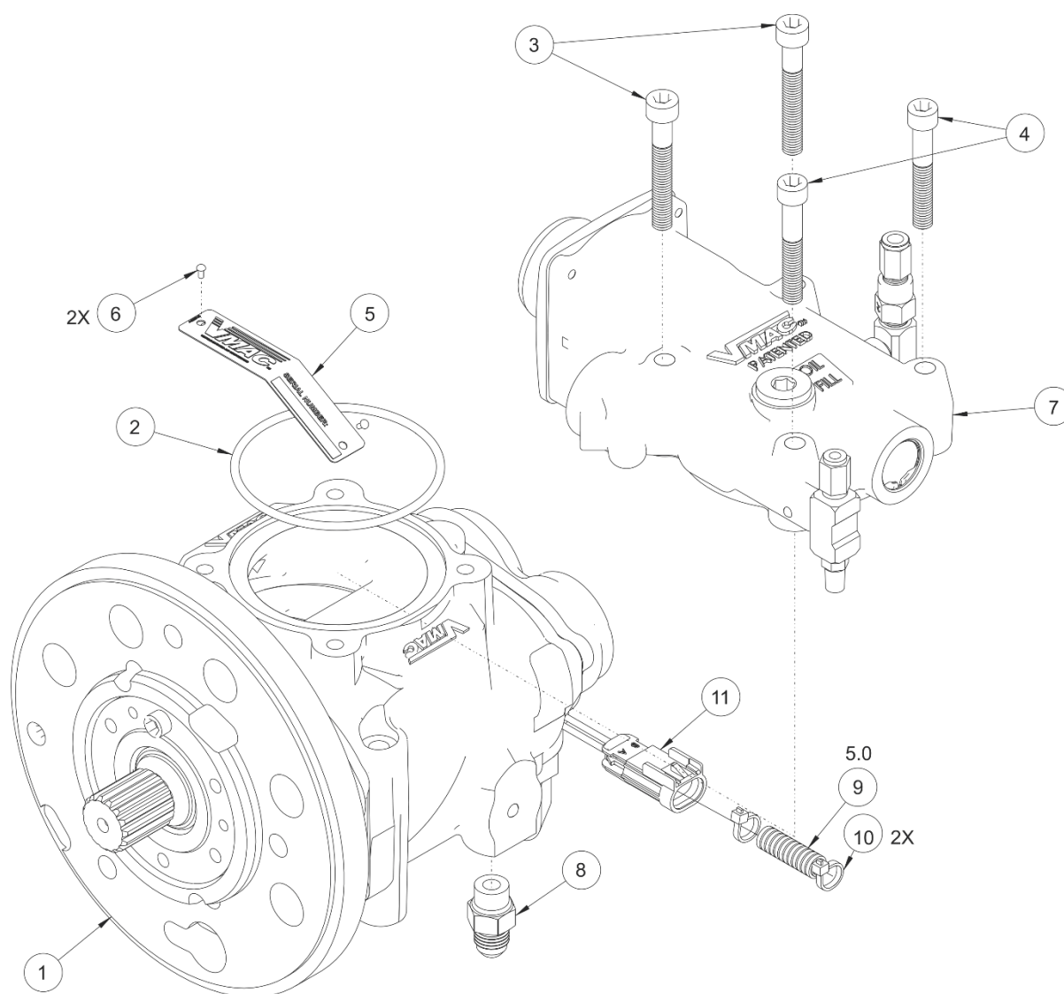
Figure 6 – Compressor Assembly
