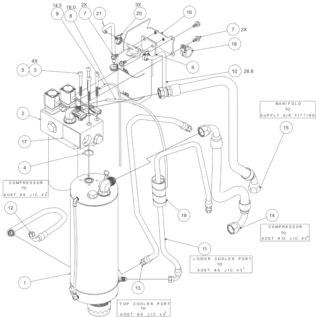
Figure 8 – Air/Oil Separator Complete Assembly
