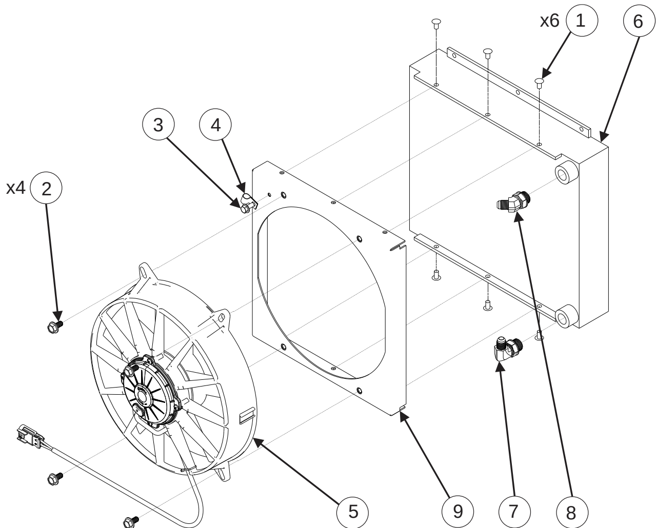
Figure 2 – Cooler Assembly
