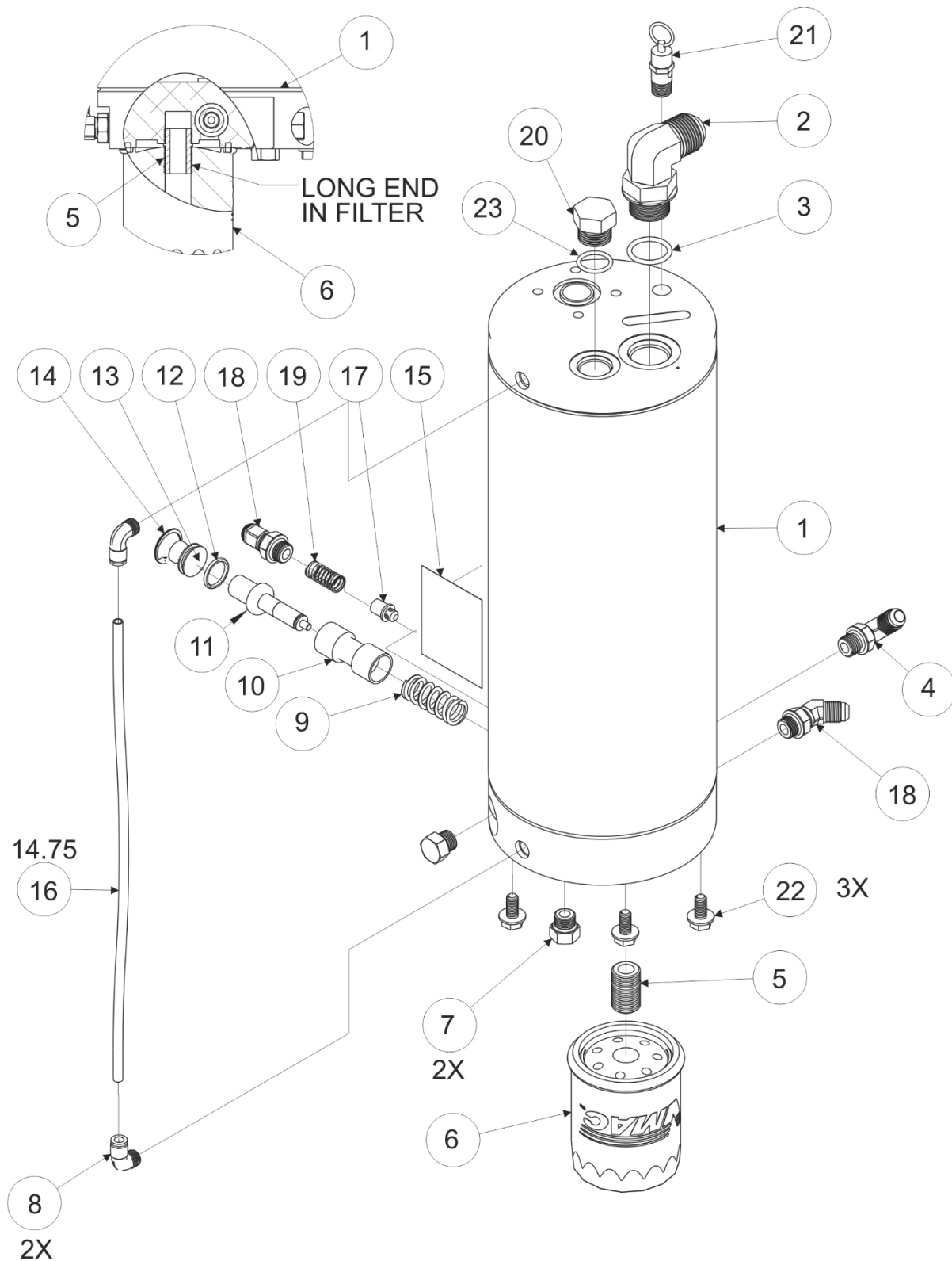
Figure 10 –Air/Oil Separator Assembly
