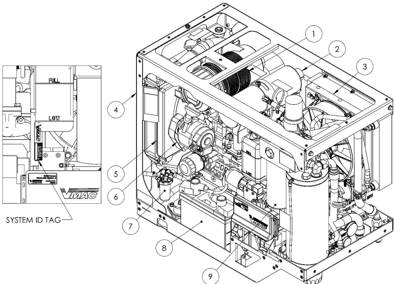
Figure 1 – Main Assembly
