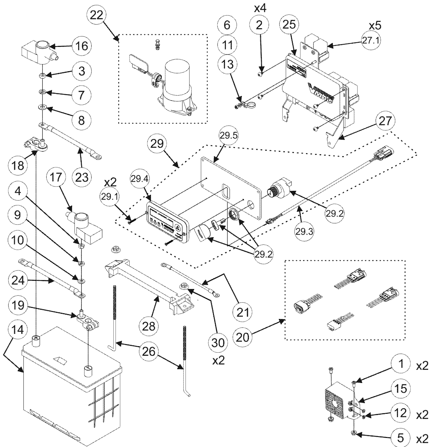
Figure 12 – D600003 and D600004 Electrical Control & System Assembly
