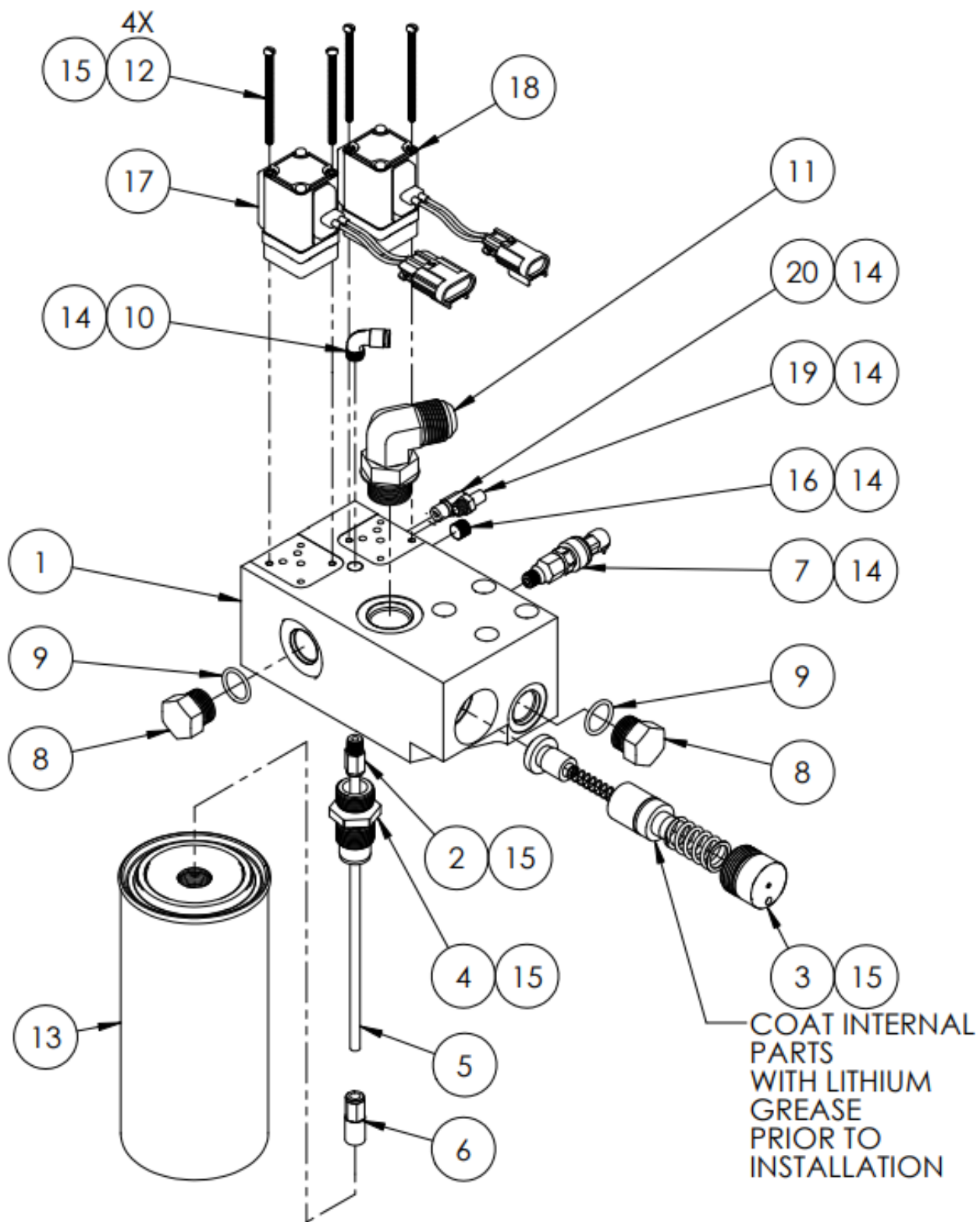
Figure 9 – Manifold Assembly
