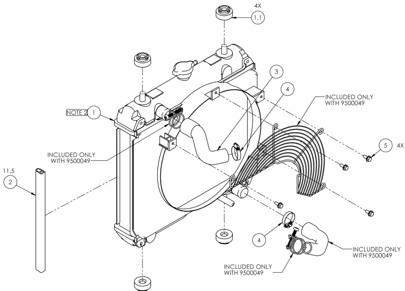
Figure 3 – Radiator Assembly
