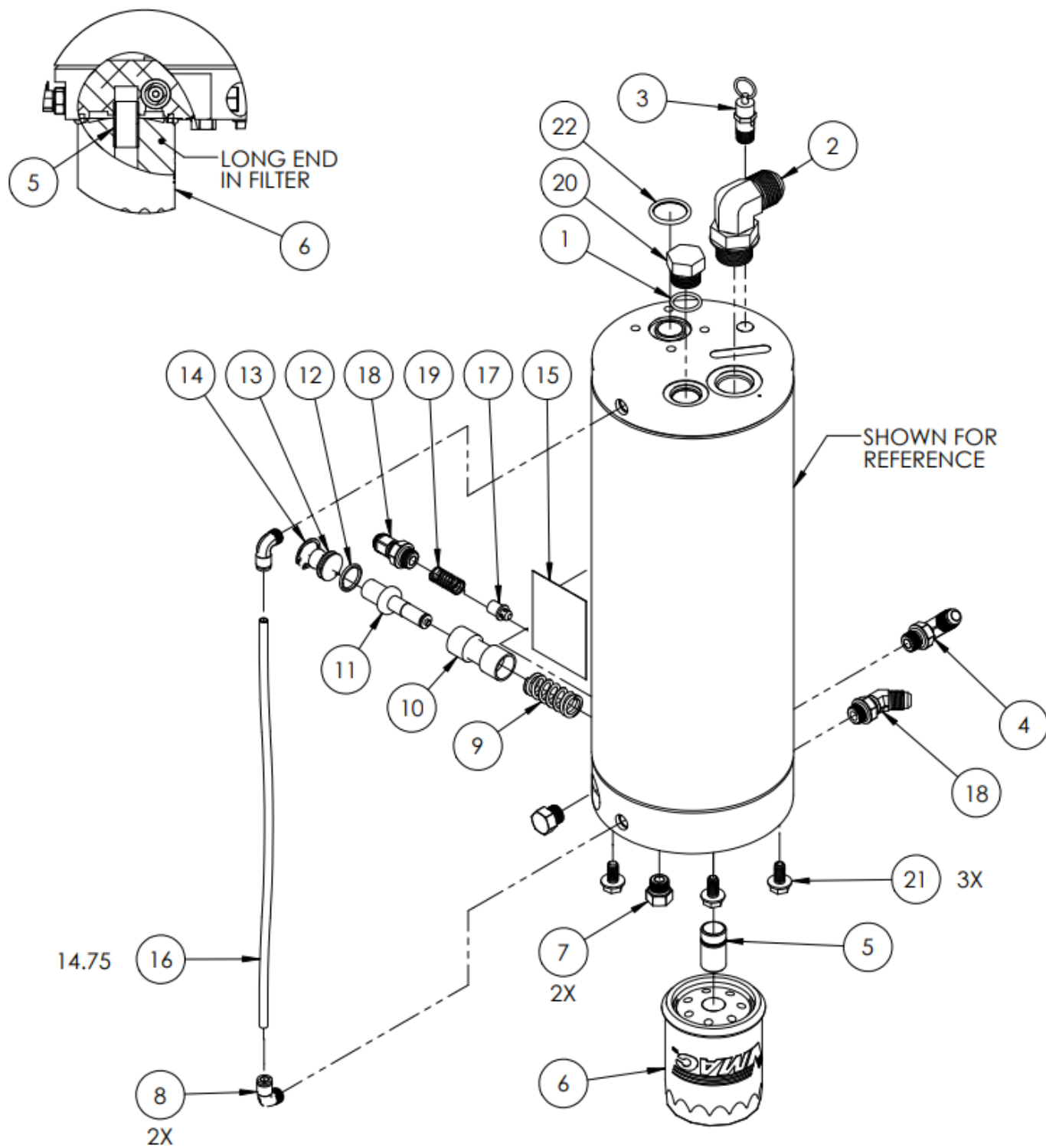
Figure 10 –Air/Oil Separator Assembly
