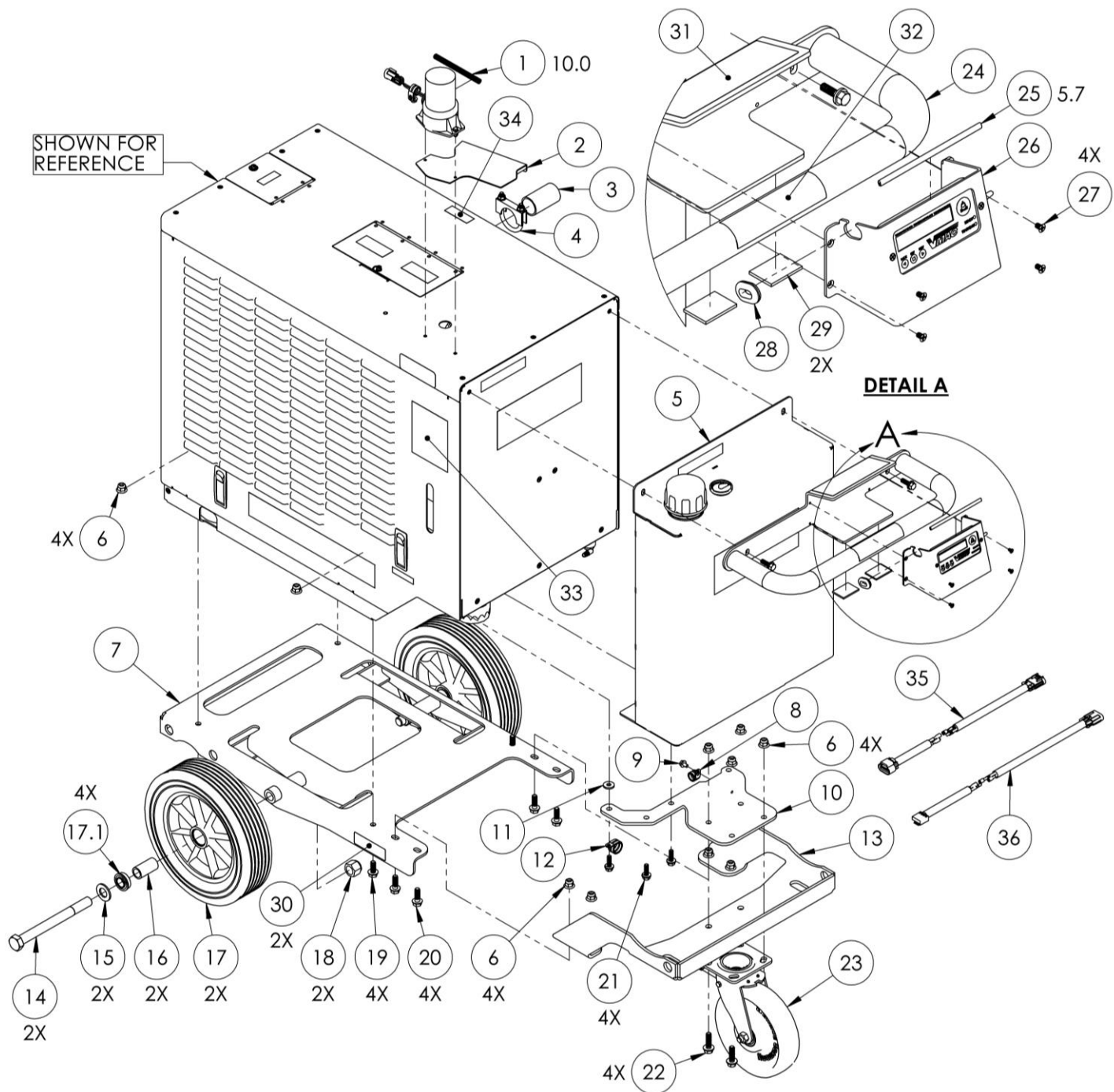
Figure 18 – D60X003 & D60X004 Wheel Kit Assembly
