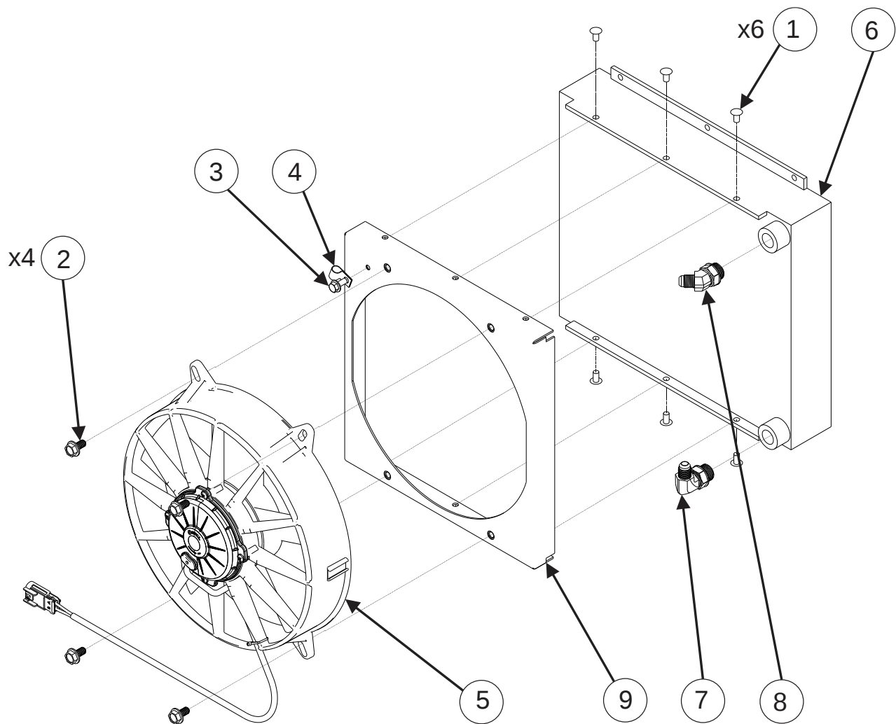
Figure 2 – Cooler Assembly
