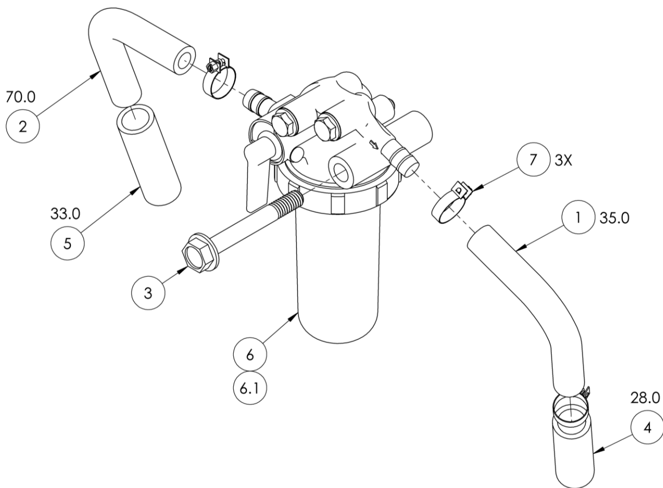
Figure 14 – Fuel Filter Assembly
