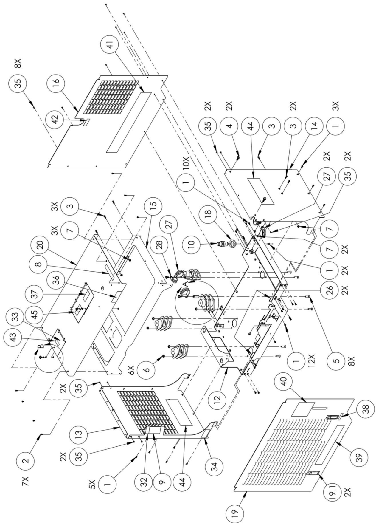
Figure 4 – Frame & Sheet Metal Assembly
