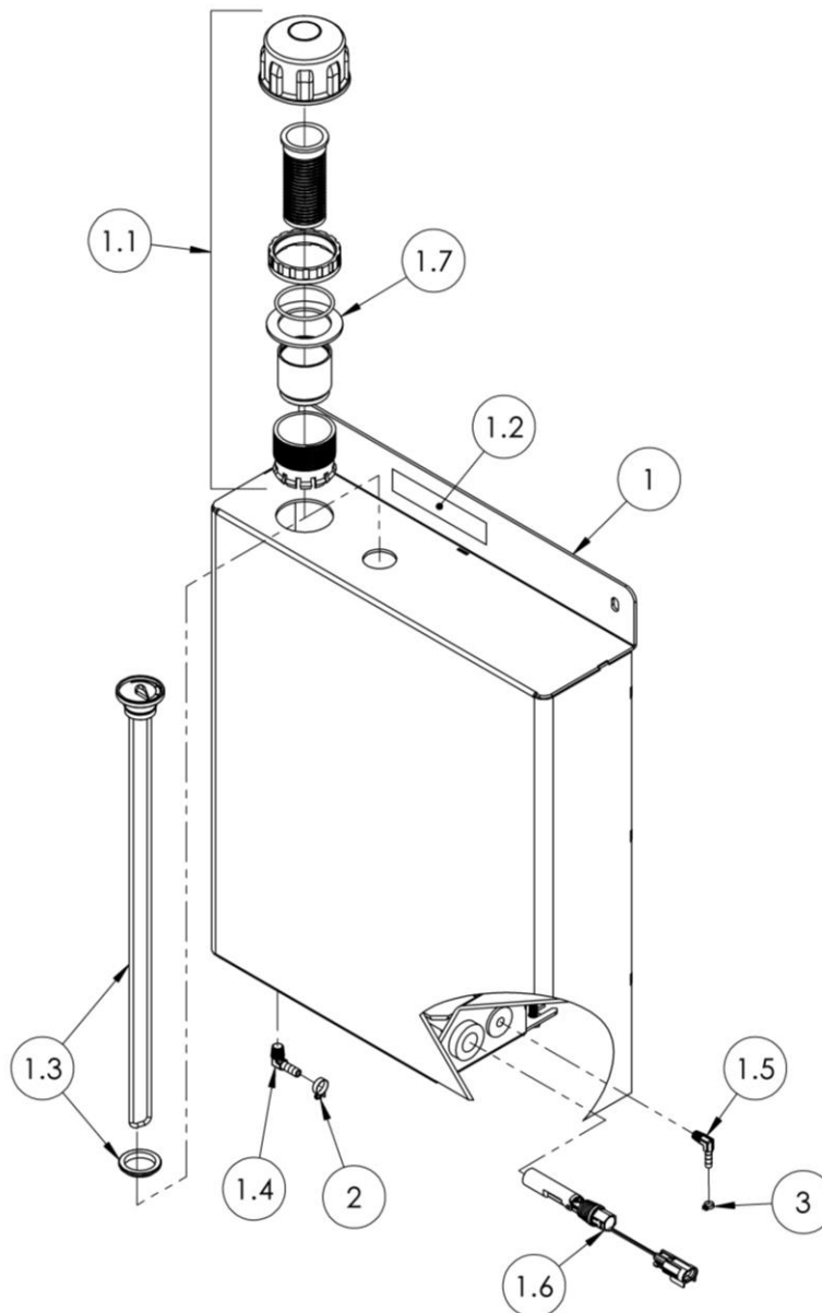
Figure 15 – Optional Fuel Tank Assembly
