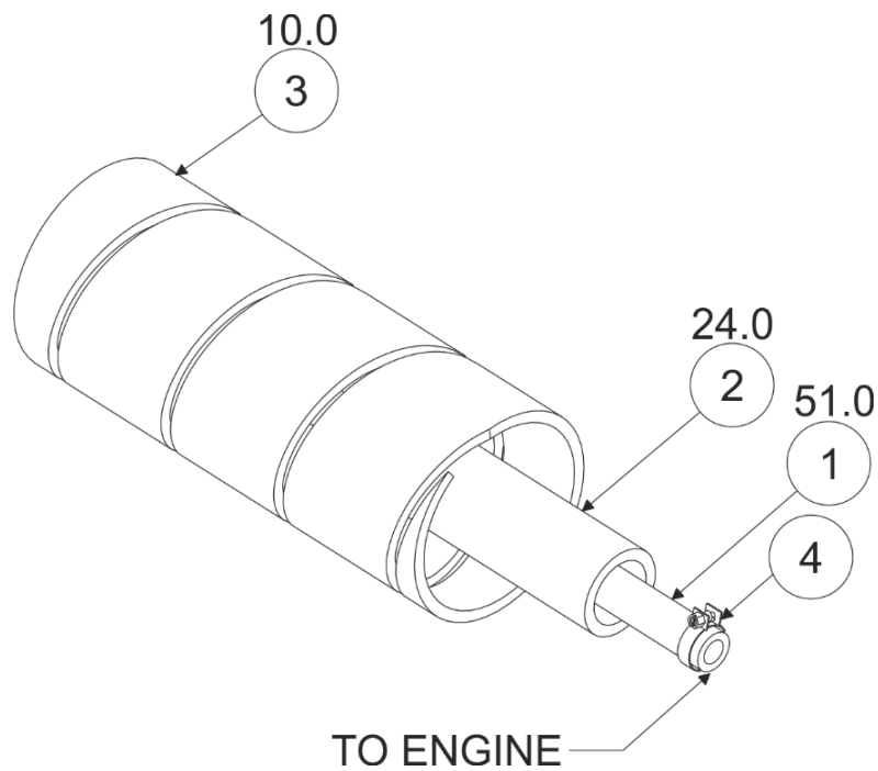
Figure 14.1 – Fuel Return Line Assembly
