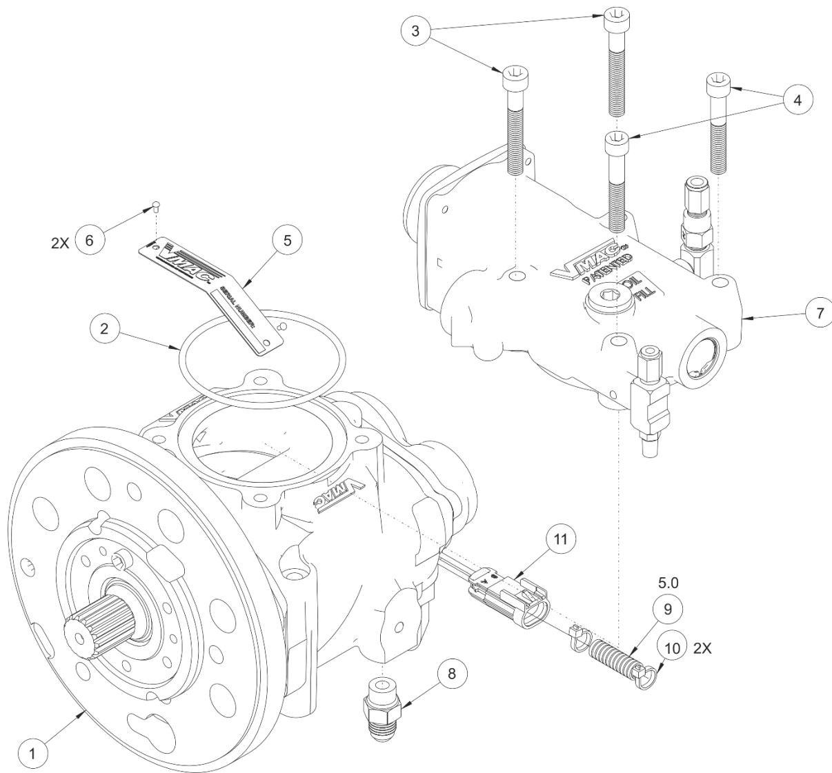
Figure 6 – Compressor Assembly
