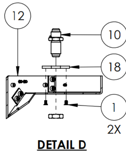
Figure 4.1 – Frame & Sheet Metal Assembly Details
