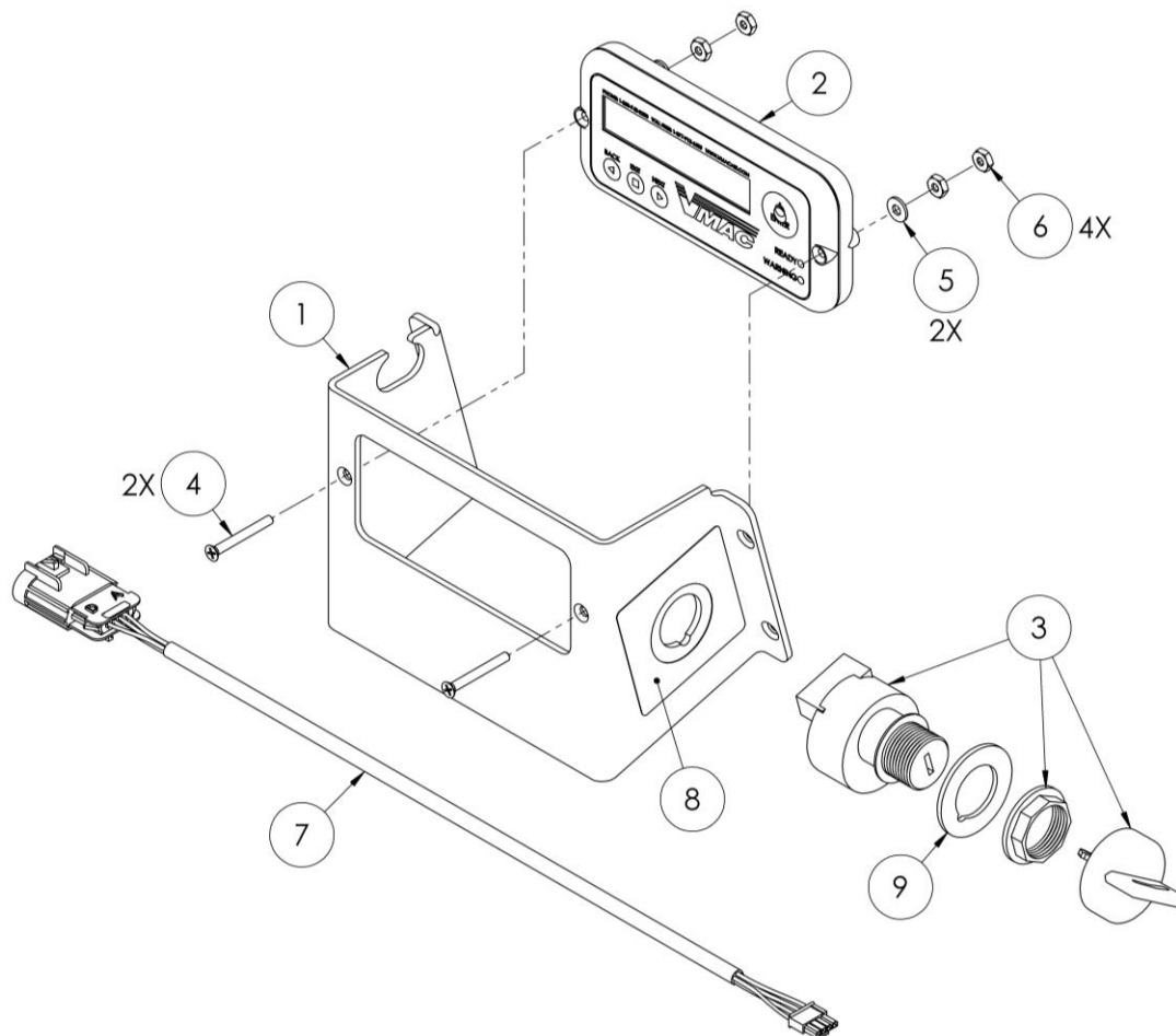
Figure 17 – D60X003 & D60X004 Display Box and Key Switch Assembly
