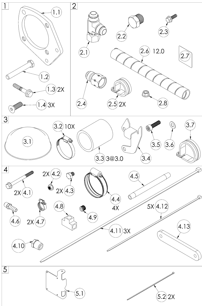
Figure 2 – Fastener Pack
