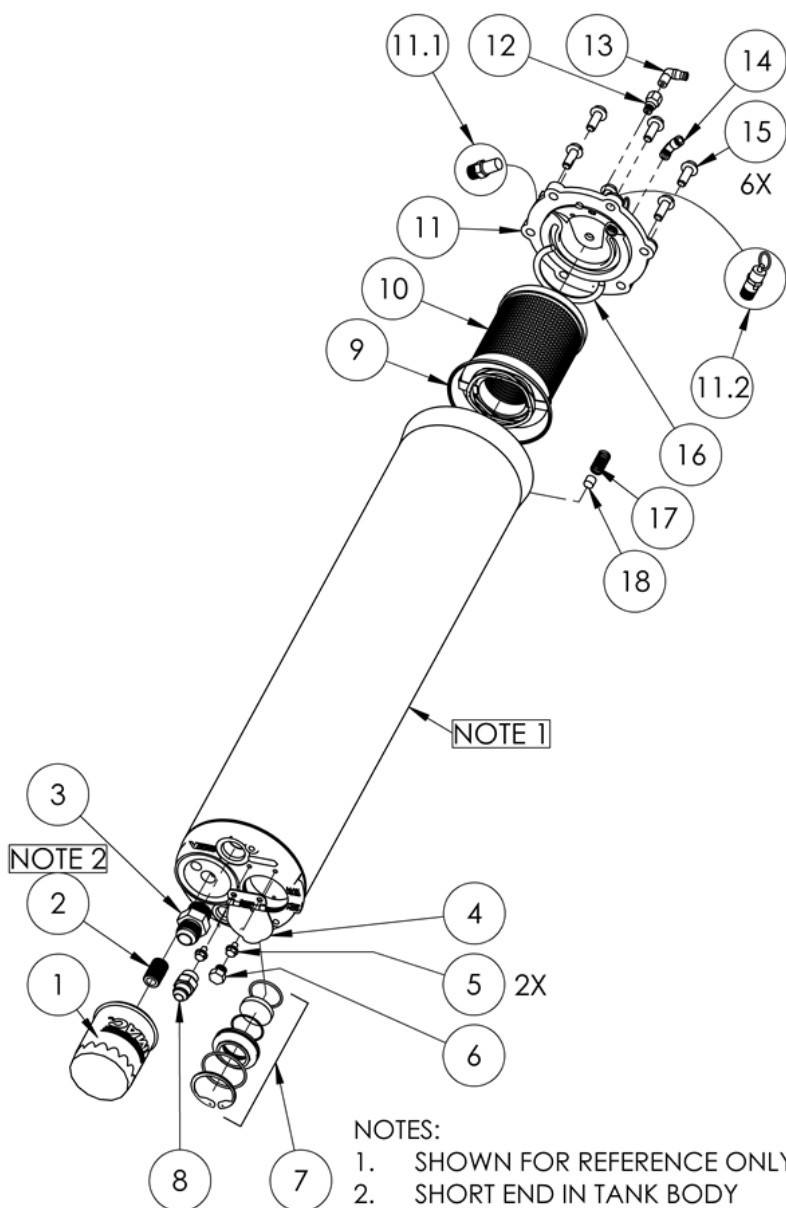
Figure 7 - VR70 Tank
