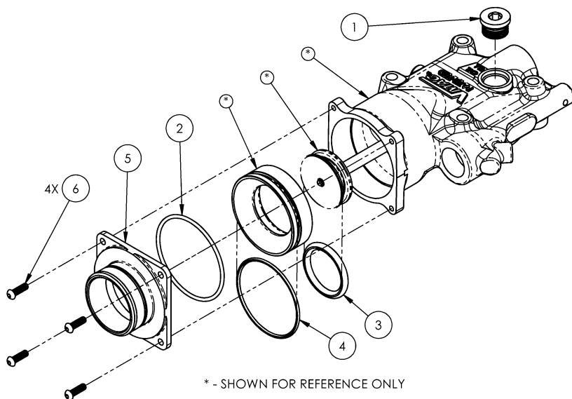
Figure 5 – Inlet Valve Sub Components
