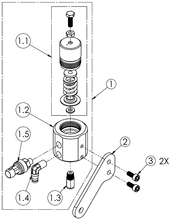
Figure 6 – Regulator & Oil Fill Components
