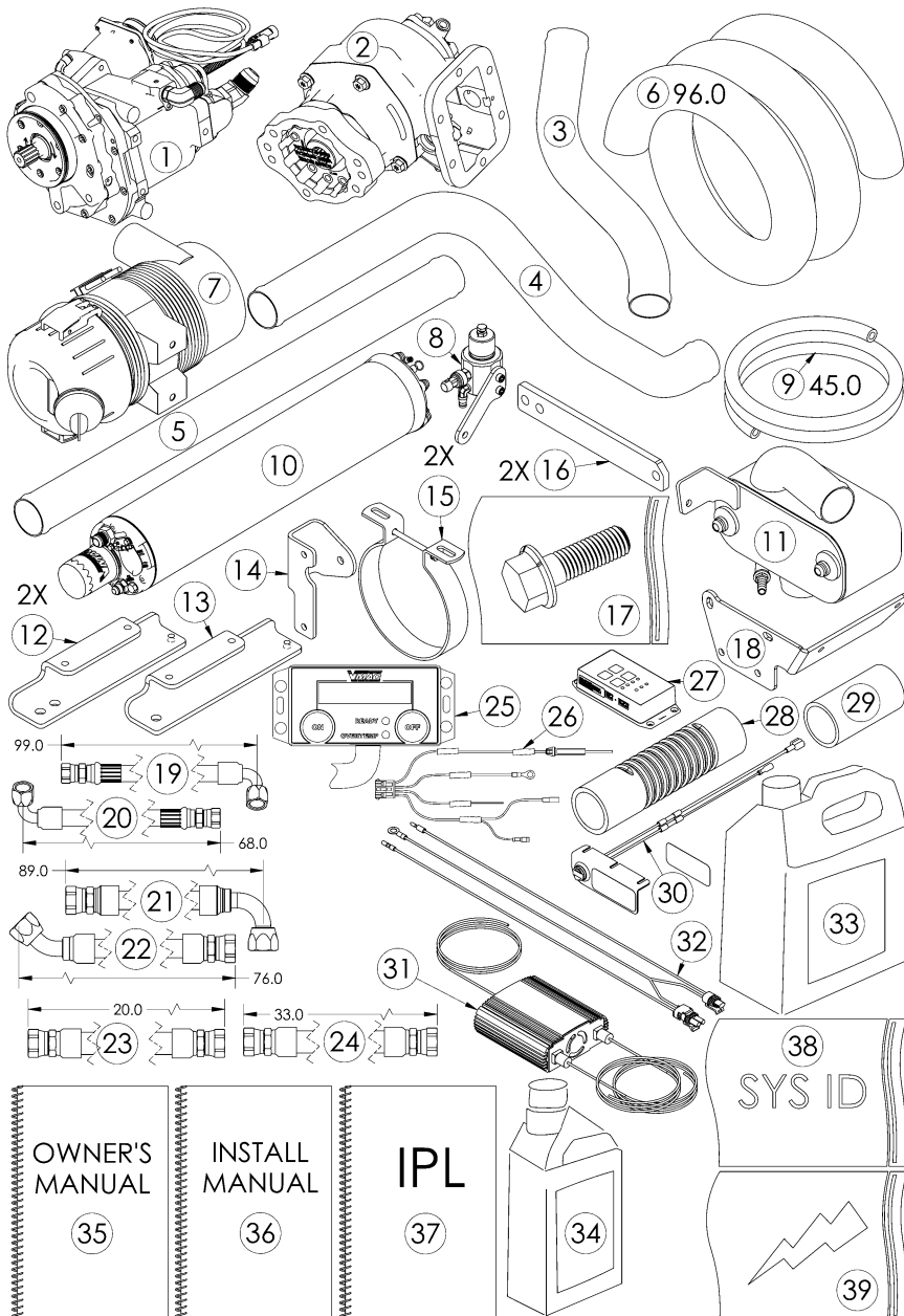
Figure 1 - Kit Pack List
