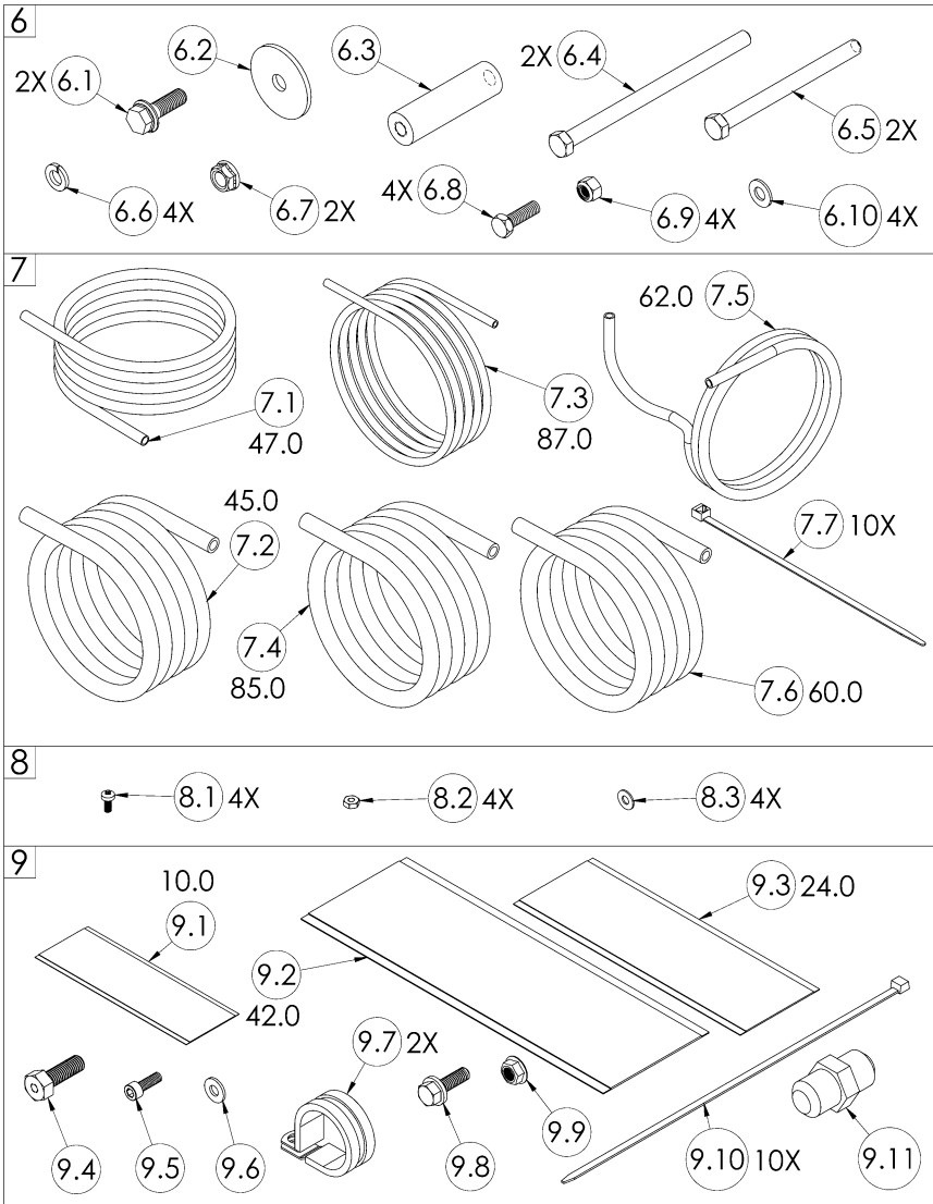
Figure 3 - Fastener Pack (cont.)
