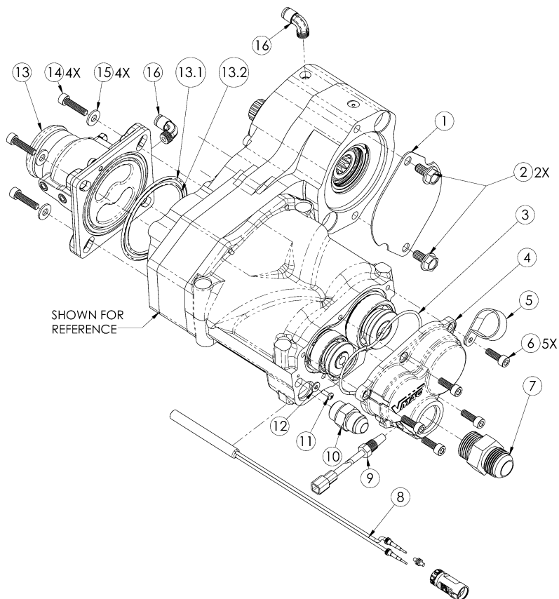
Figure 4 - Compressor Assembly
