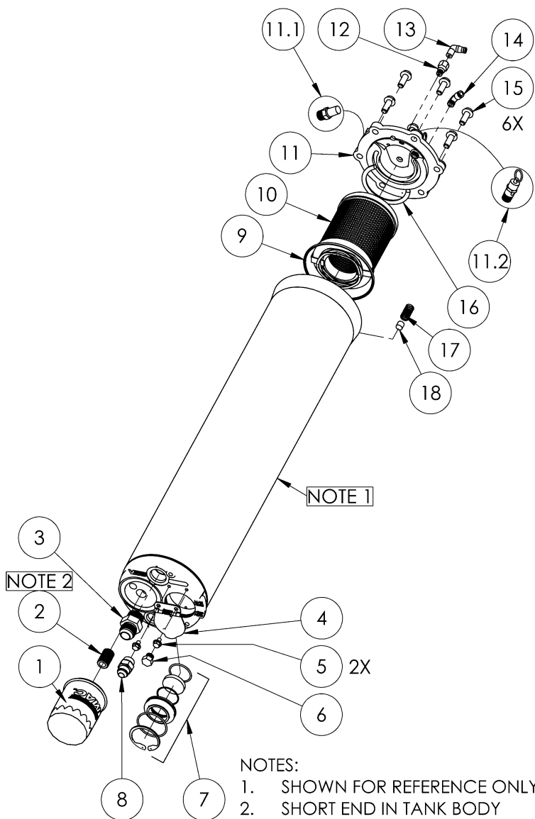
Figure 7 - VR70 Tank
