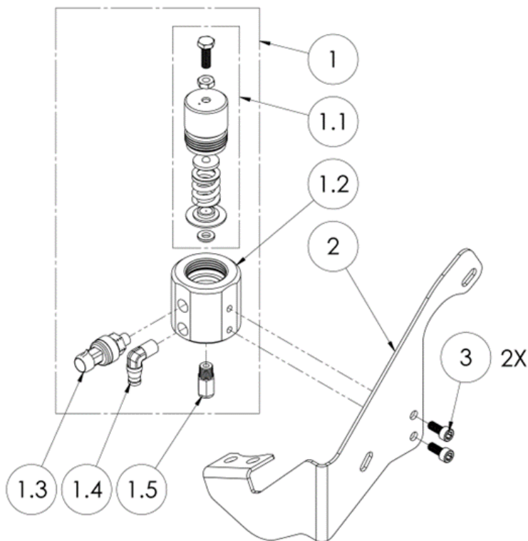
Figure 5 - Regulator Sub Components
