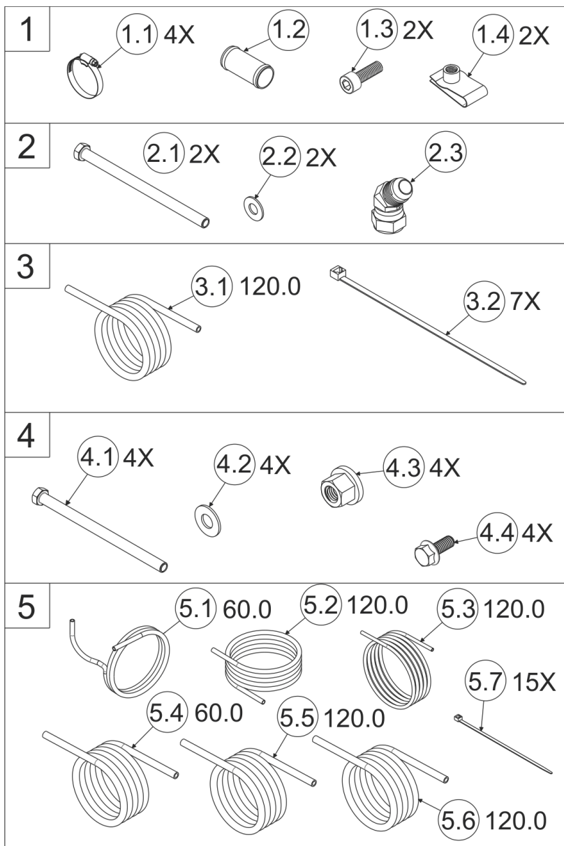
Figure 2 - Fastener Packs
