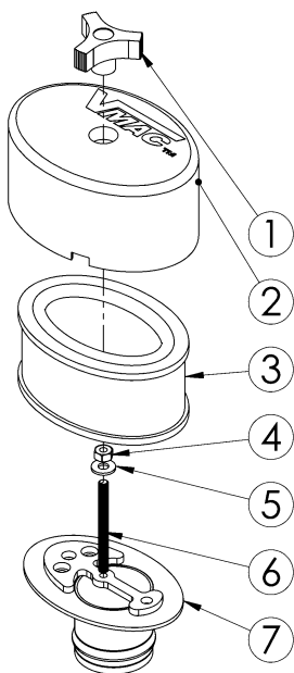
Figure 6 – Air Filter Sub Components
