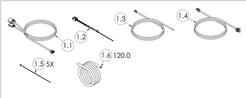
Figure 8 – Electrical Pack, 3810107
