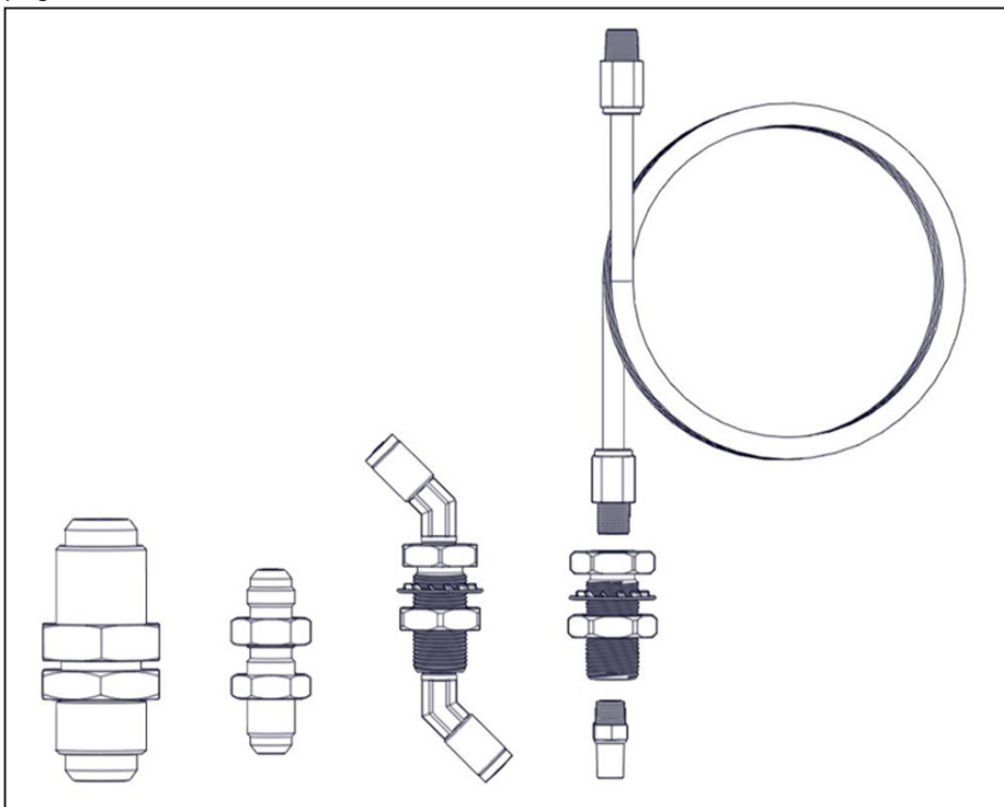
Figure 32 — Bulkhead fittings
