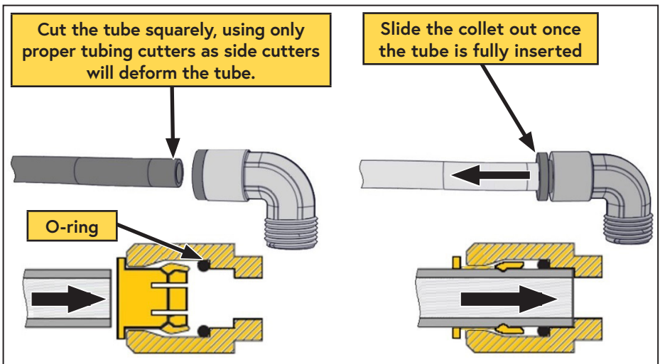
Figure 37 — Push-to-connect fittings
