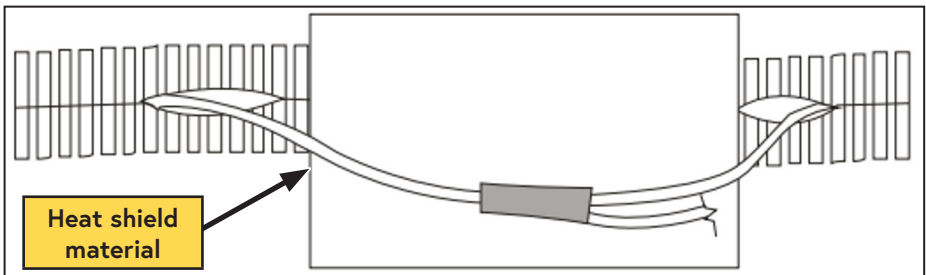
Figure 30 — Seal soldered joint
