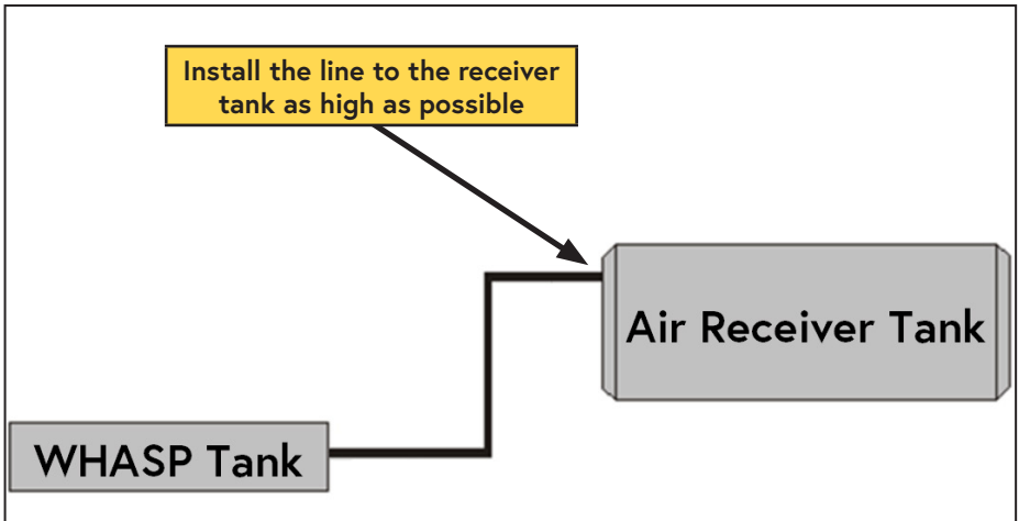
Figure 45 — Air receiver tank
