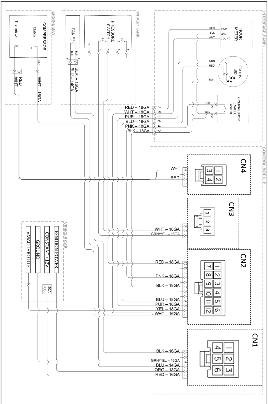
Figure 36 — Electrical schematic
