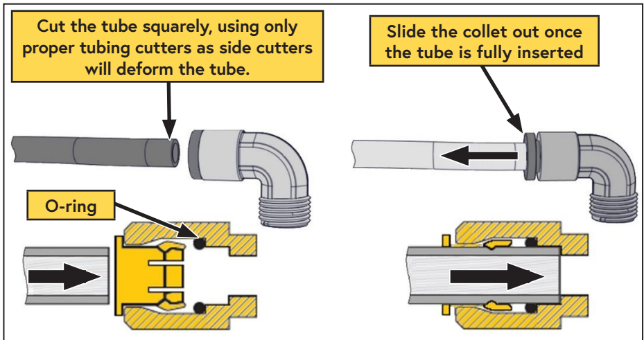
Figure 26 — Push-to-connect fittings
