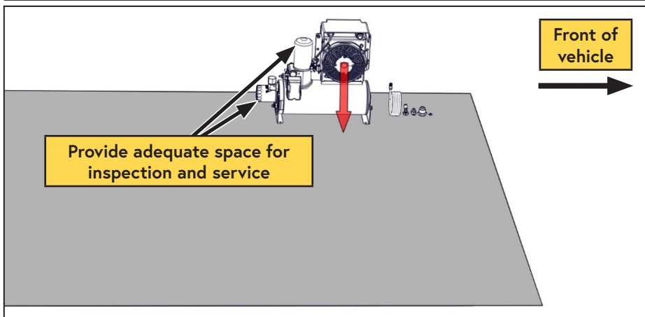
Figure 24 — WHASP ventilation
