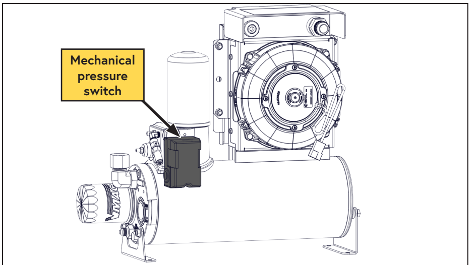
Figure 35 — WHASP Tank pressure switch
