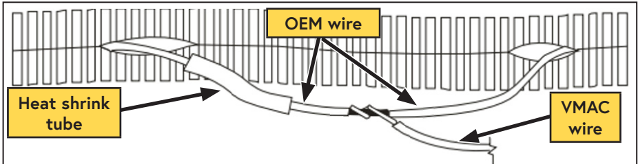
Figure 29 — Solder spliced joint
