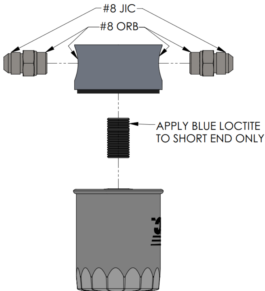
Figure 1 – Remote Oil Filter Assembly Instructions
